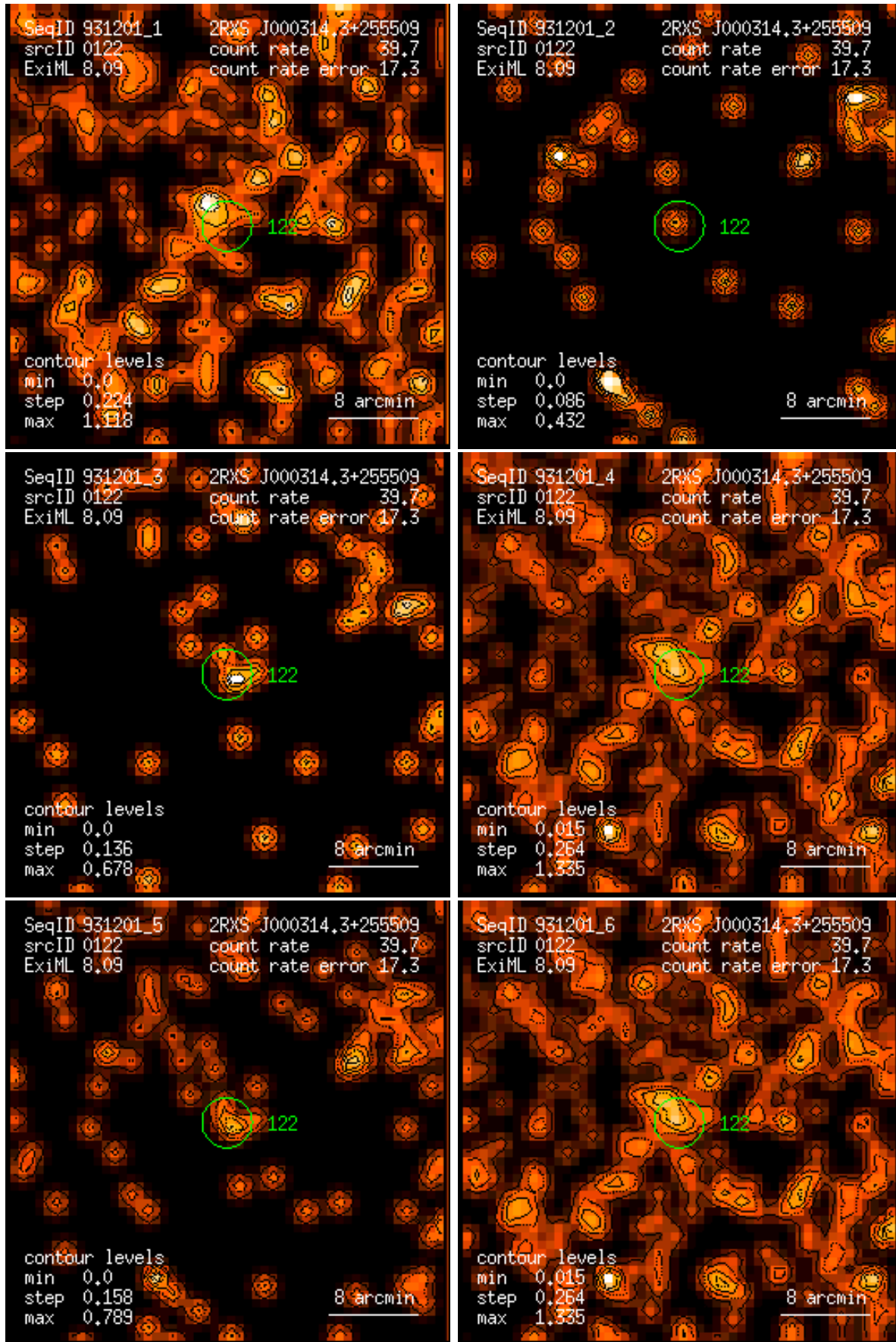
Figure 122: RASS 931201: detection 0122: band rate images, Gaussian filter: (1) PSPC channels 11 – 41, (2) 52 – 90, (3) 91 – 201, (4) 11 – 235, (5) 52 – 201, (6) 11 – 201. Broad band rates in counts/ks. Band rate contour levels in counts/ks/arcmin 2 .
