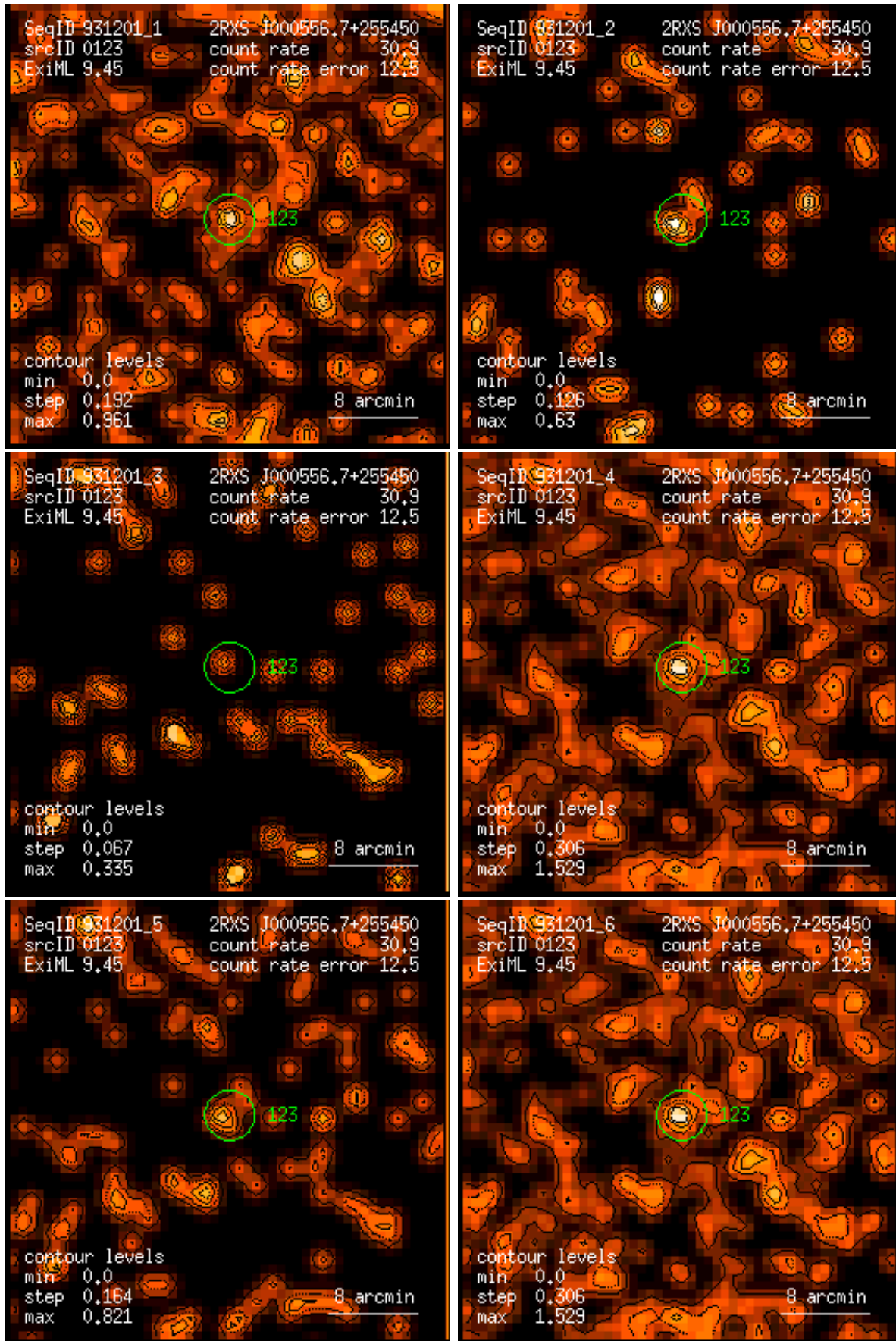
Figure 123: RASS 931201: detection 0123: band rate images, Gaussian filter: (1) PSPC channels 11 – 41, (2) 52 – 90, (3) 91 – 201, (4) 11 – 235, (5) 52 – 201, (6) 11 – 201. Broad band rates in counts/ks. Band rate contour levels in counts/ks/arcmin 2 .
