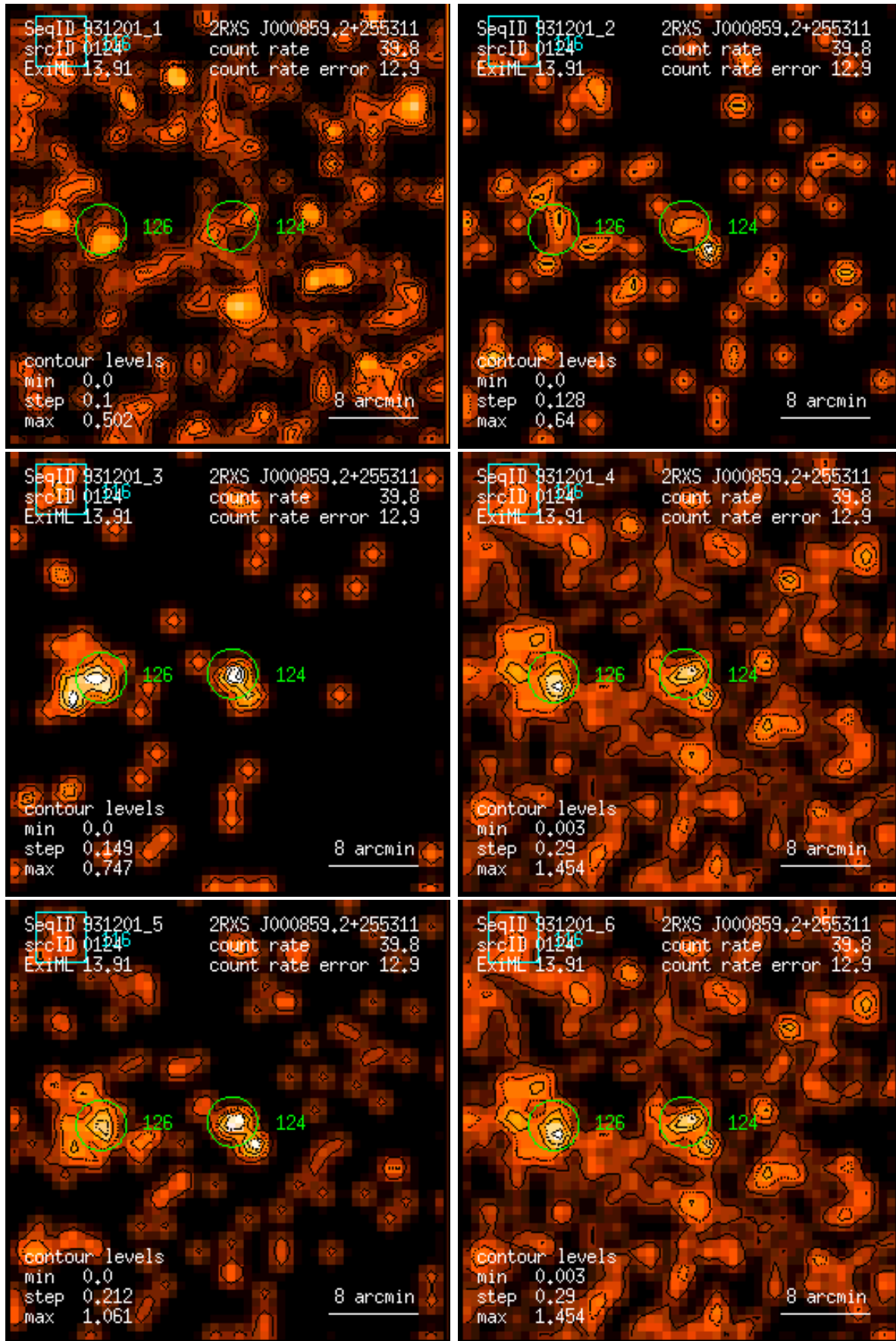
Figure 124: RASS 931201: detection 0124: band rate images, Gaussian filter: (1) PSPC channels 11 – 41, (2) 52 – 90, (3) 91 – 201, (4) 11 – 235, (5) 52 – 201, (6) 11 – 201. Broad band rates in counts/ks. Band rate contour levels in counts/ks/arcmin 2 .
