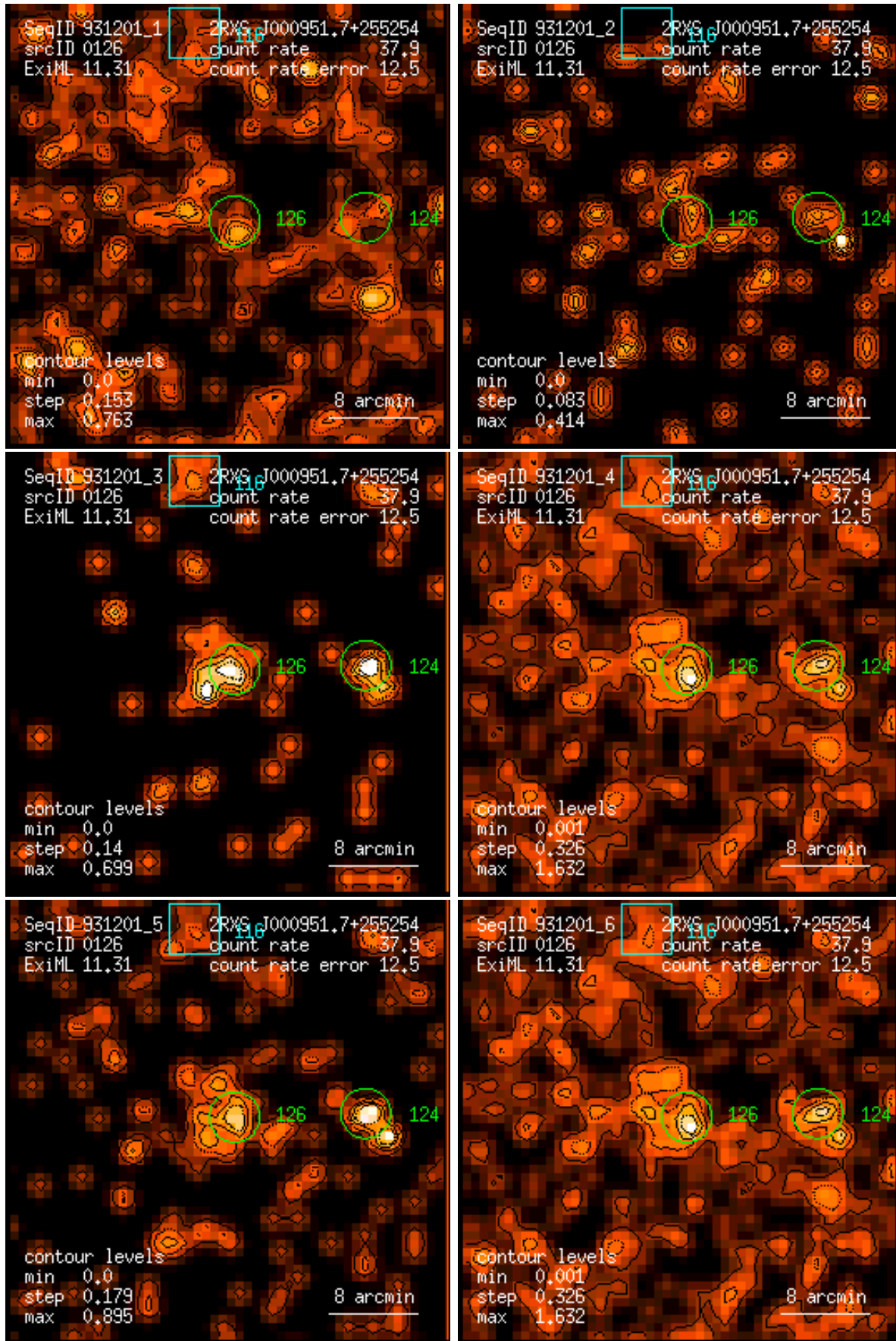
Figure 126: RASS 931201: detection 0126: band rate images, Gaussian filter: (1) PSPC channels 11 – 41, (2) 52 – 90, (3) 91 – 201, (4) 11 – 235, (5) 52 – 201, (6) 11 – 201. Broad band rates in counts/ks. Band rate contour levels in counts/ks/arcmin 2 .
