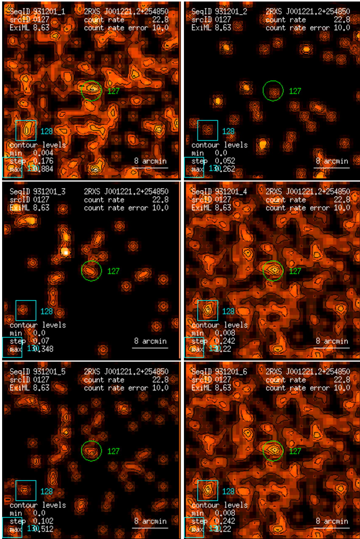
Figure 127: RASS 931201: detection 0127: band rate images, Gaussian filter: (1) PSPC channels 11 – 41, (2) 52 – 90, (3) 91 – 201, (4) 11 – 235, (5) 52 – 201, (6) 11 – 201. Broad band rates in counts/ks. Band rate contour levels in counts/ks/arcmin 2 .
