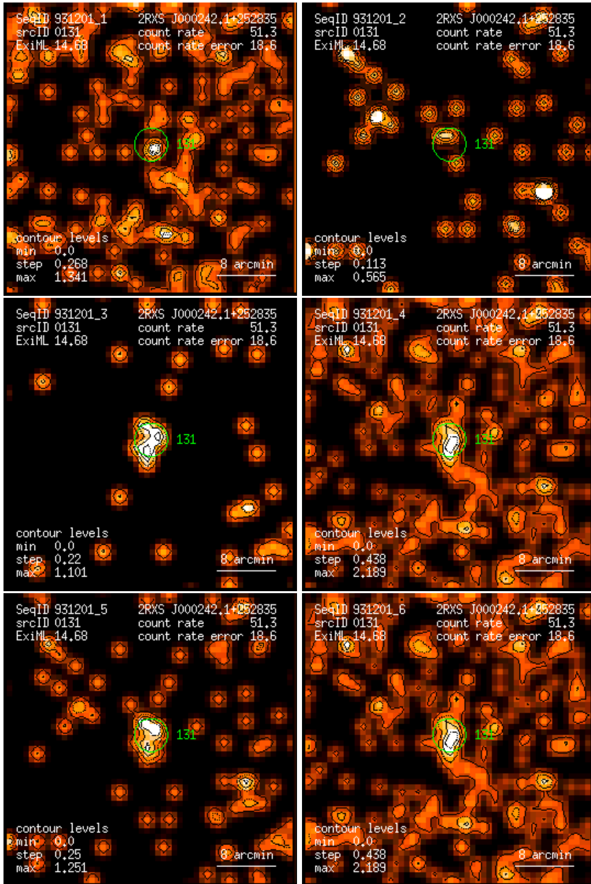
Figure 131: RASS 931201: detection 0131: band rate images, Gaussian filter: (1) PSPC channels 11 – 41, (2) 52 – 90, (3) 91 – 201, (4) 11 – 235, (5) 52 – 201, (6) 11 – 201. Broad band rates in counts/ks. Band rate contour levels in counts/ks/arcmin 2 .
