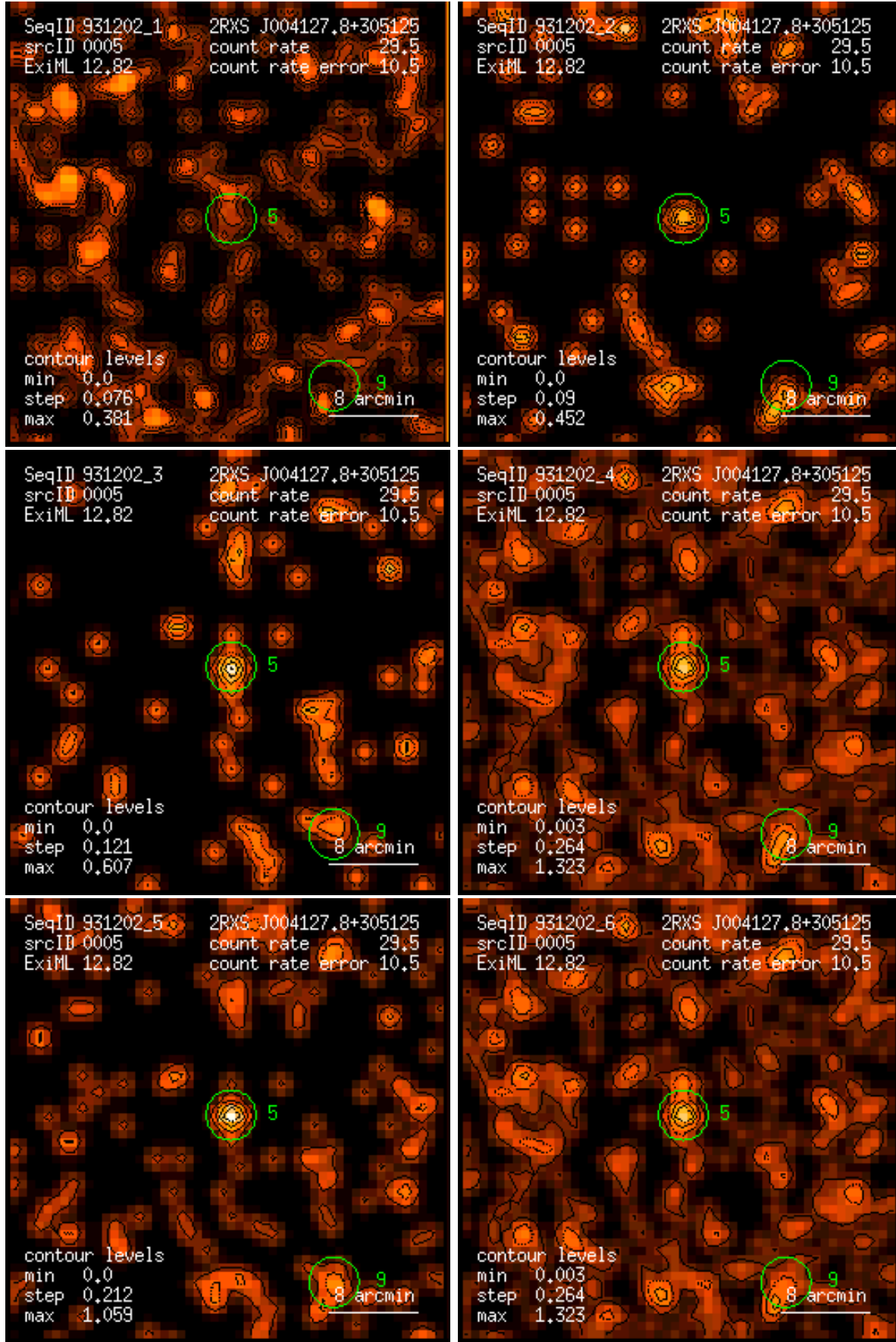
Figure 5: RASS 931202: detection 0005: band rate images, Gaussian filter: (1) PSPC channels 11 – 41, (2) 52 – 90, (3) 91 – 201, (4) 11 – 235, (5) 52 – 201, (6) 11 – 201. Broad band rates in counts/ks. Band rate contour levels in counts/ks/arcmin 2 .
