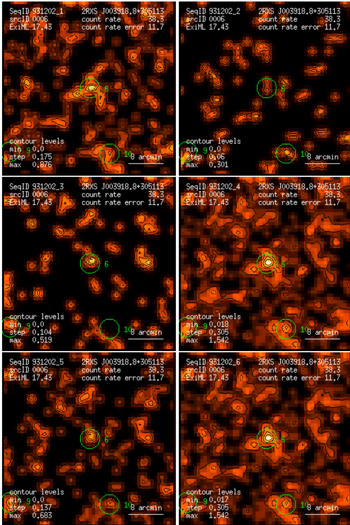
Figure 6: RASS 931202: detection 0006: band rate images, Gaussian filter: (1) PSPC channels 11 – 41, (2) 52 – 90, (3) 91 – 201, (4) 11 – 235, (5) 52 – 201, (6) 11 – 201. Broad band rates in counts/ks. Band rate contour levels in counts/ks/arcmin 2 .
