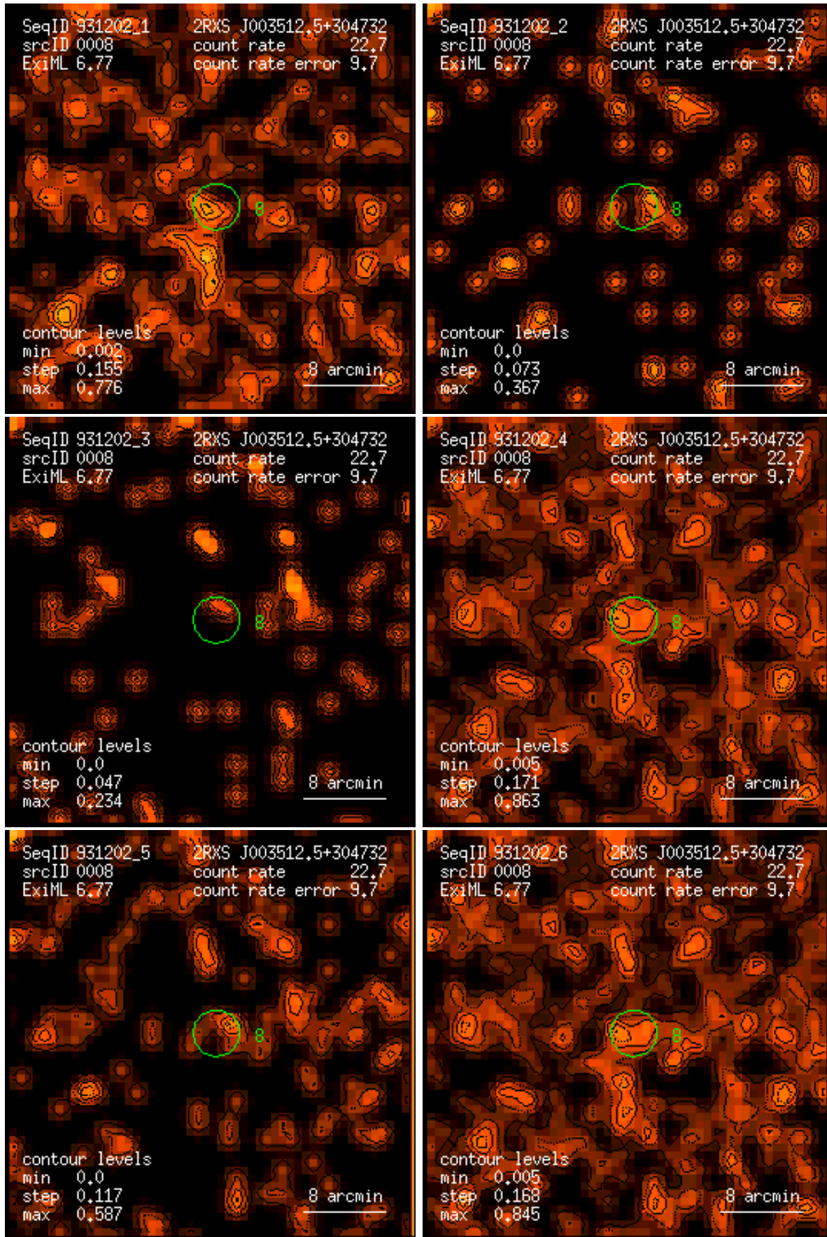
Figure 8: RASS 931202: detection 0008: band rate images, Gaussian filter: (1) PSPC channels 11 – 41, (2) 52 – 90, (3) 91 – 201, (4) 11 – 235, (5) 52 – 201, (6) 11 – 201. Broad band rates in counts/ks. Band rate contour levels in counts/ks/arcmin 2 .
