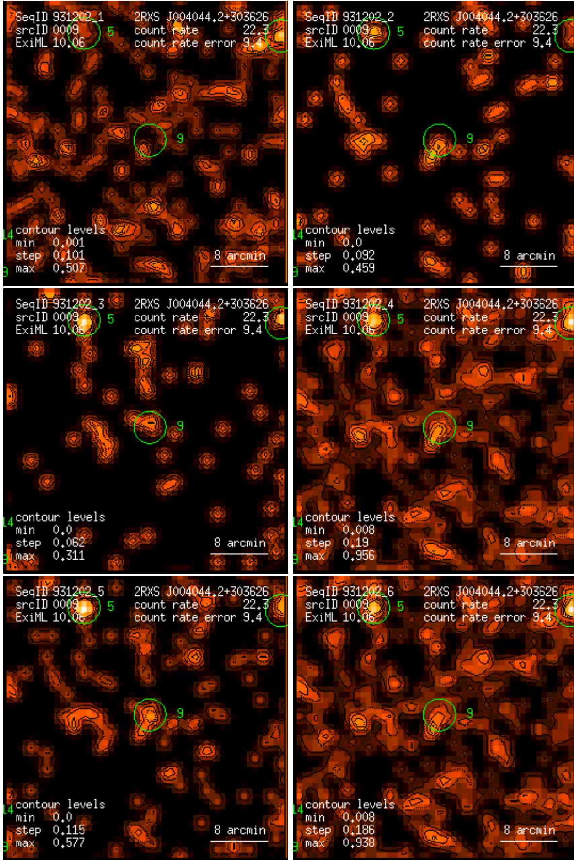
Figure 9: RASS 931202: detection 0009: band rate images, Gaussian filter: (1) PSPC channels 11 – 41, (2) 52 – 90, (3) 91 – 201, (4) 11 – 235, (5) 52 – 201, (6) 11 – 201. Broad band rates in counts/ks. Band rate contour levels in counts/ks/arcmin 2 .
