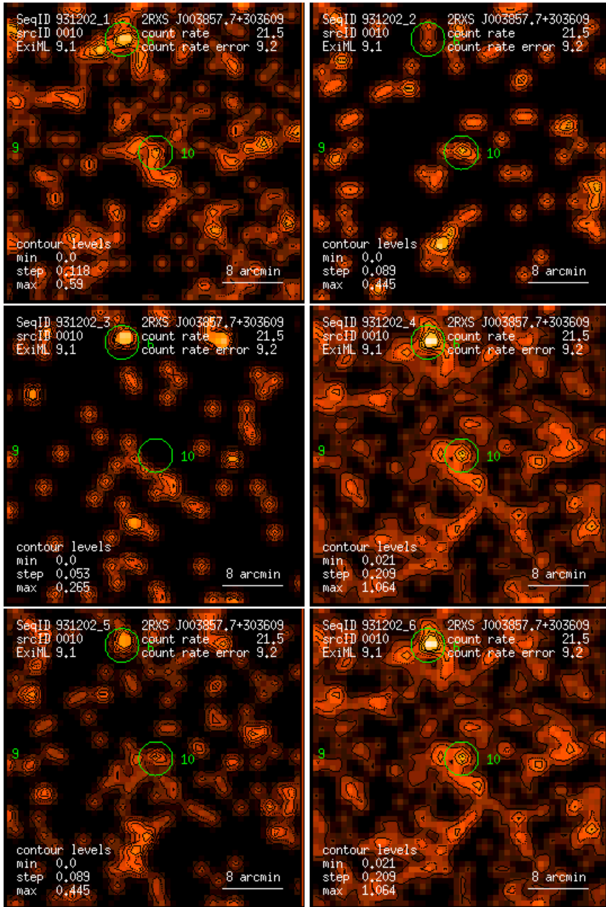
Figure 10: RASS 931202: detection 0010: band rate images, Gaussian filter: (1) PSPC channels 11 – 41, (2) 52 – 90, (3) 91 – 201, (4) 11 – 235, (5) 52 – 201, (6) 11 – 201. Broad band rates in counts/ks. Band rate contour levels in counts/ks/arcmin 2 .
