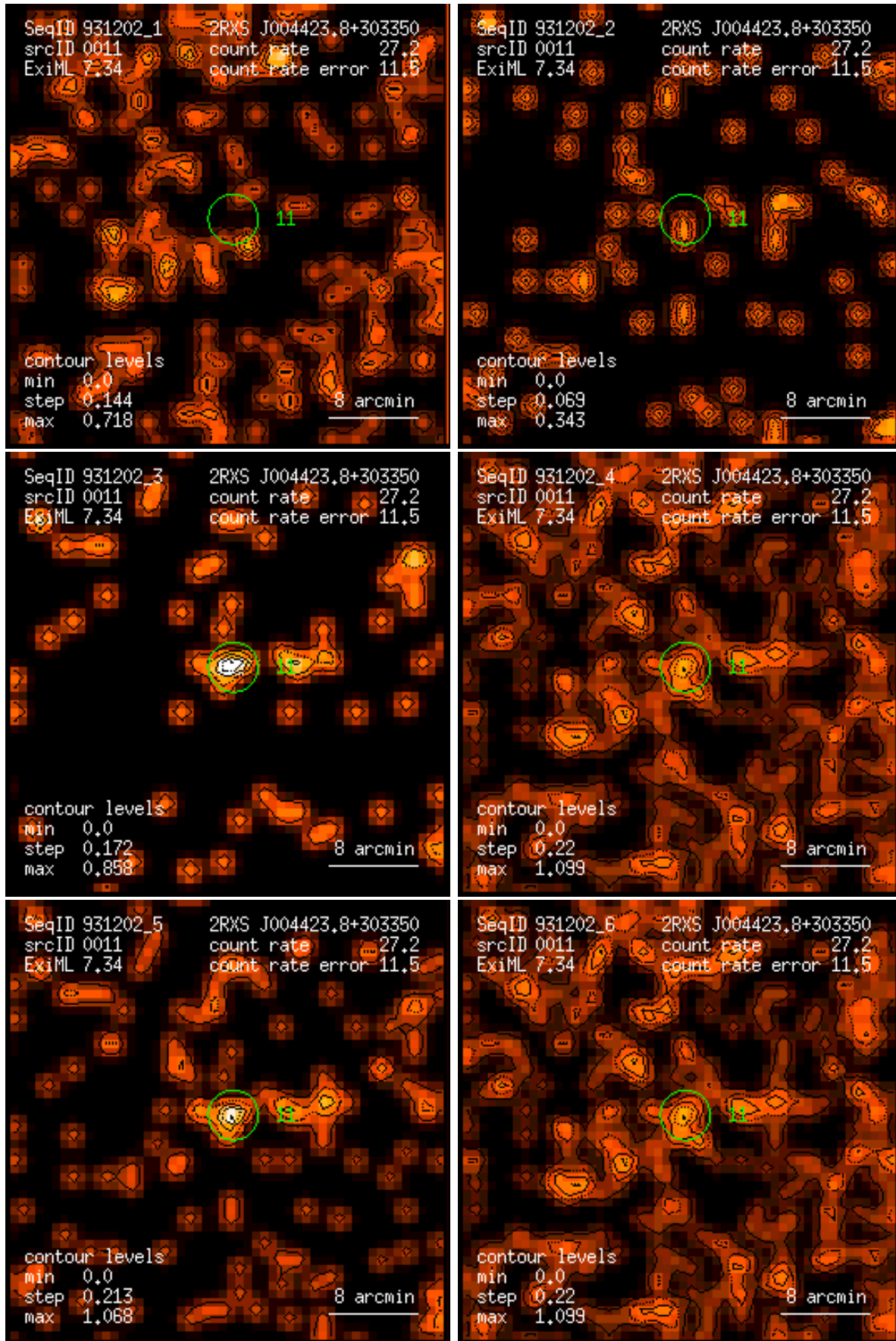
Figure 11: RASS 931202: detection 0011: band rate images, Gaussian filter: (1) PSPC channels 11 – 41, (2) 52 – 90, (3) 91 – 201, (4) 11 – 235, (5) 52 – 201, (6) 11 – 201. Broad band rates in counts/ks. Band rate contour levels in counts/ks/arcmin 2 .
