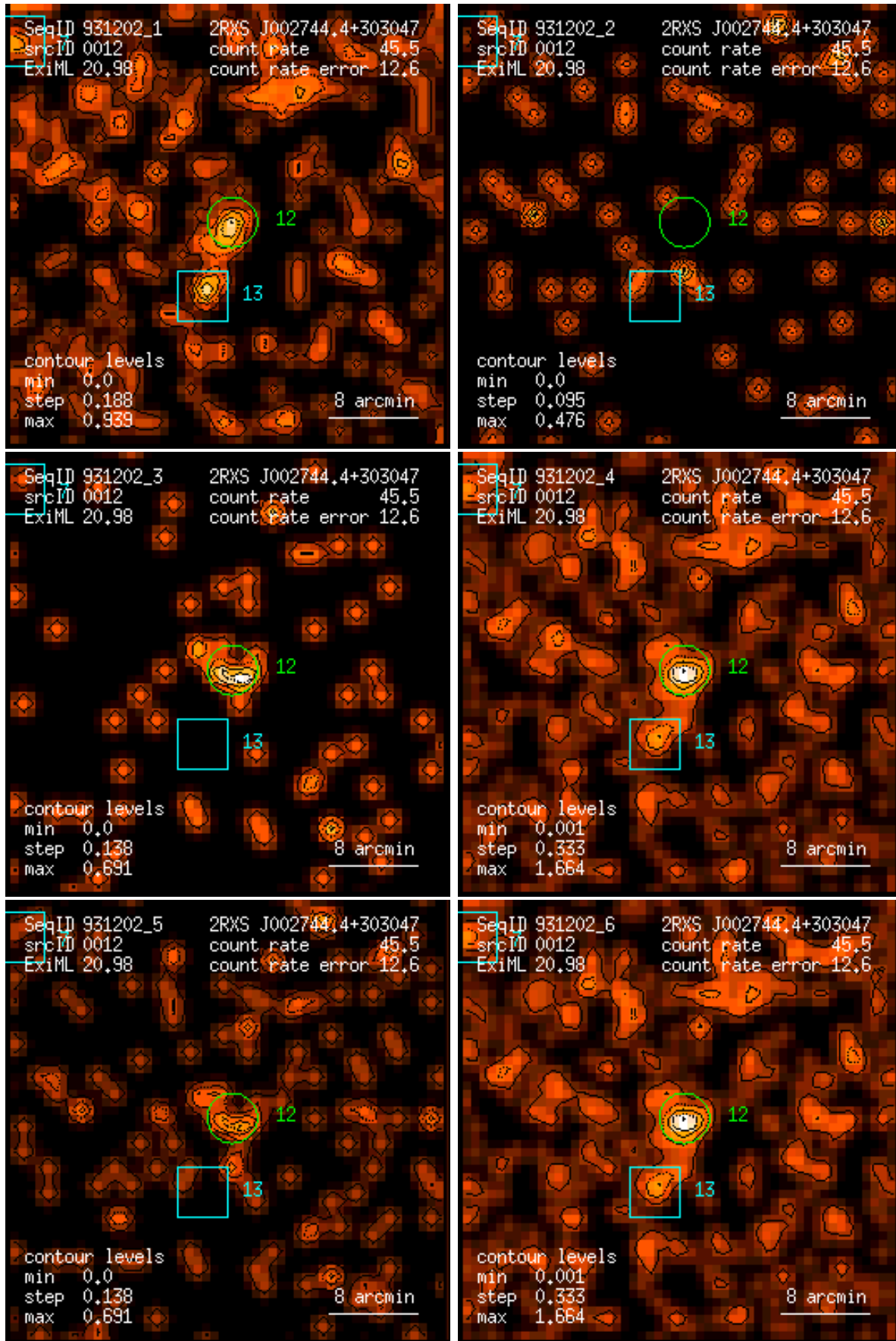
Figure 12: RASS 931202: detection 0012: band rate images, Gaussian filter: (1) PSPC channels 11 – 41, (2) 52 – 90, (3) 91 – 201, (4) 11 – 235, (5) 52 – 201, (6) 11 – 201. Broad band rates in counts/ks. Band rate contour levels in counts/ks/arcmin 2 .
