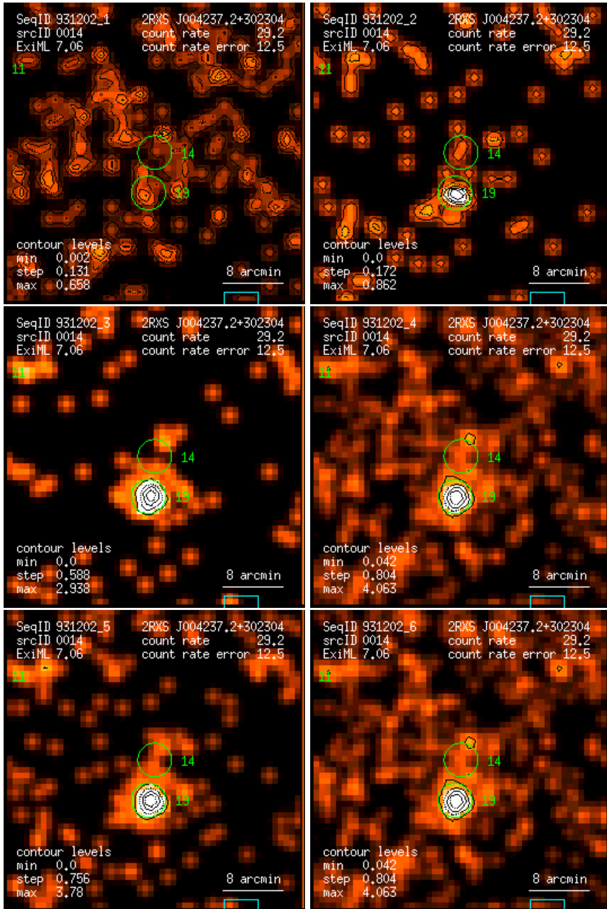
Figure 14: RASS 931202: detection 0014: band rate images, Gaussian filter: (1) PSPC channels 11 – 41, (2) 52 – 90, (3) 91 – 201, (4) 11 – 235, (5) 52 – 201, (6) 11 – 201. Broad band rates in counts/ks. Band rate contour levels in counts/ks/arcmin 2 .
