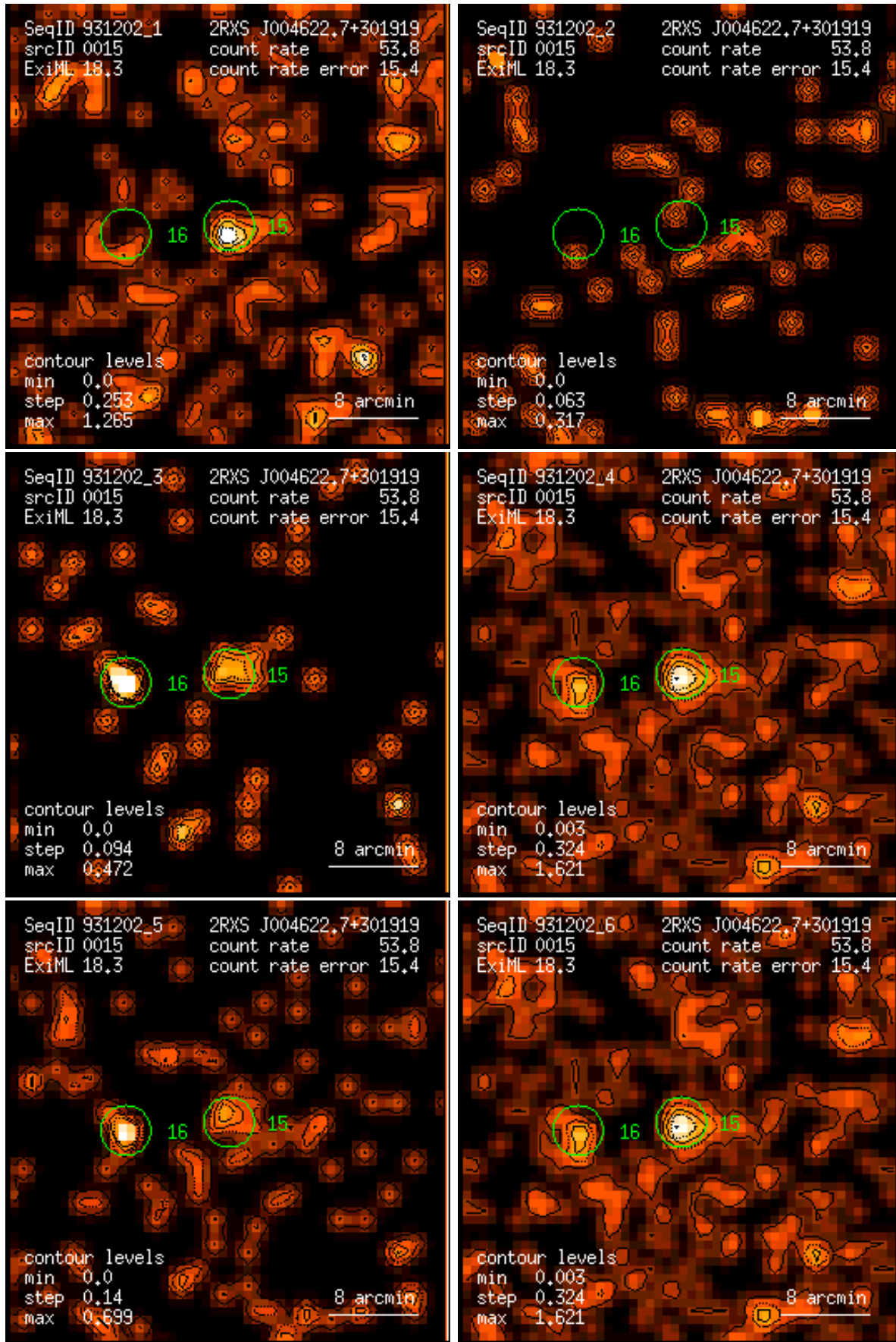
Figure 15: RASS 931202: detection 0015: band rate images, Gaussian filter: (1) PSPC channels 11 – 41, (2) 52 – 90, (3) 91 – 201, (4) 11 – 235, (5) 52 – 201, (6) 11 – 201. Broad band rates in counts/ks. Band rate contour levels in counts/ks/arcmin 2 .
