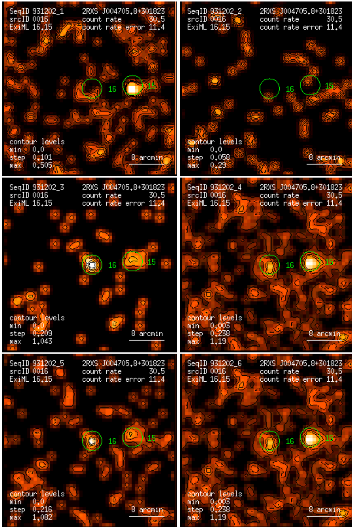
Figure 16: RASS 931202: detection 0016: band rate images, Gaussian filter: (1) PSPC channels 11 – 41, (2) 52 – 90, (3) 91 – 201, (4) 11 – 235, (5) 52 – 201, (6) 11 – 201. Broad band rates in counts/ks. Band rate contour levels in counts/ks/arcmin 2 .
