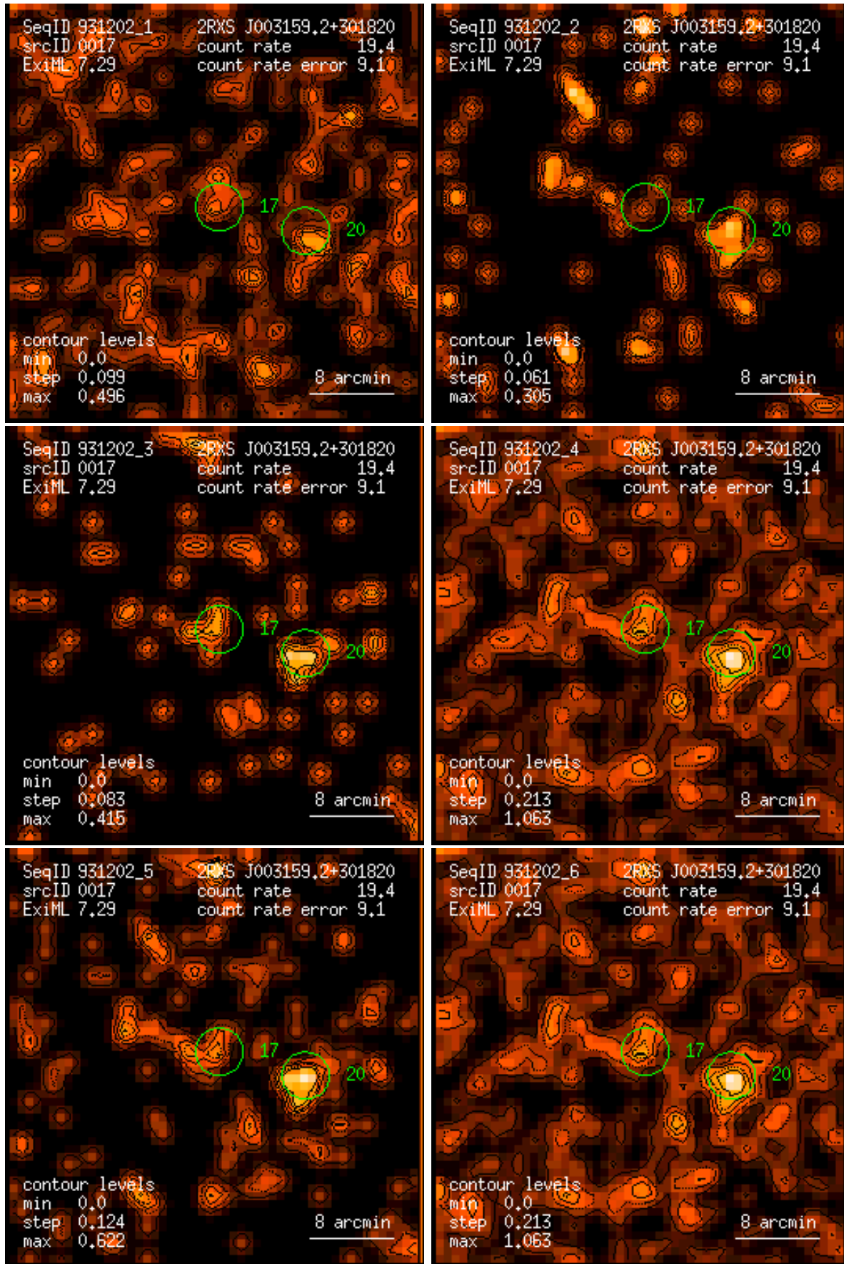
Figure 17: RASS 931202: detection 0017: band rate images, Gaussian filter: (1) PSPC channels 11 – 41, (2) 52 – 90, (3) 91 – 201, (4) 11 – 235, (5) 52 – 201, (6) 11 – 201. Broad band rates in counts/ks. Band rate contour levels in counts/ks/arcmin 2 .
