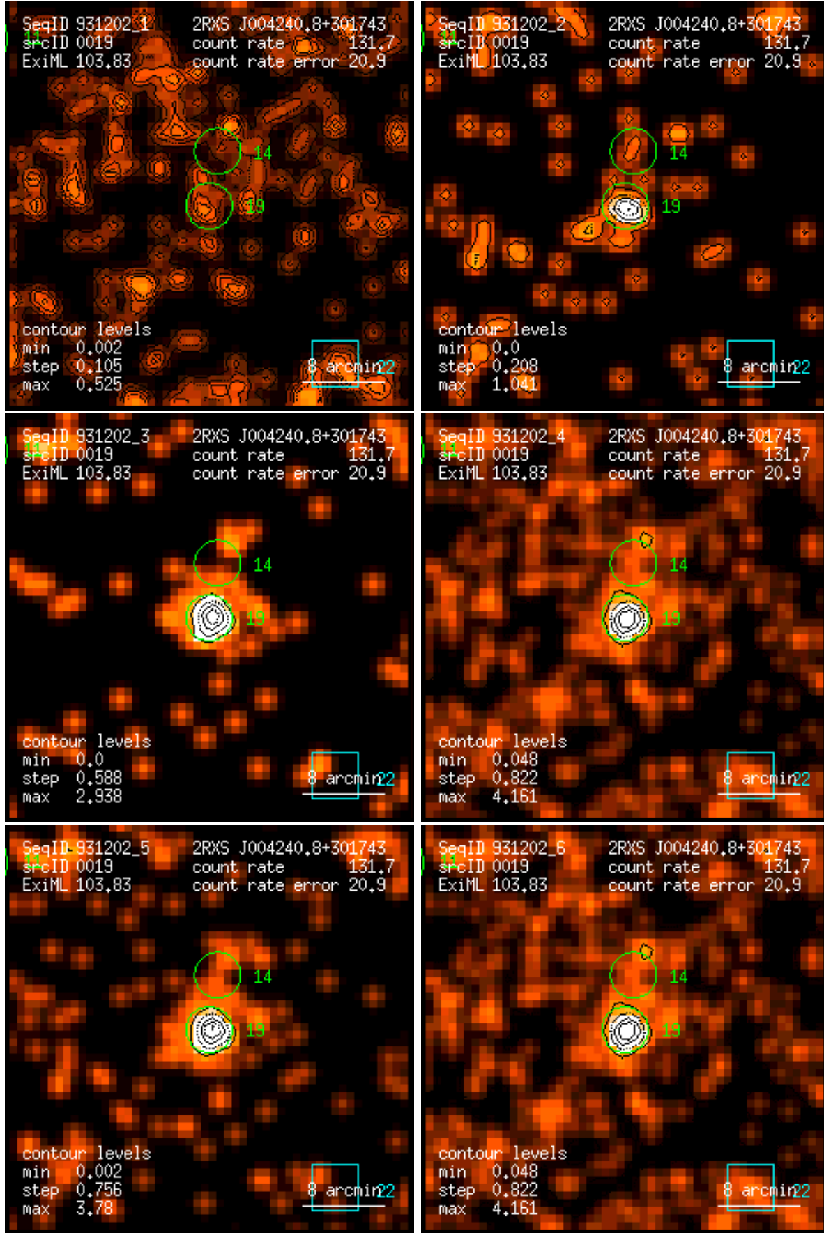
Figure 19: RASS 931202: detection 0019: band rate images, Gaussian filter: (1) PSPC channels 11 – 41, (2) 52 – 90, (3) 91 – 201, (4) 11 – 235, (5) 52 – 201, (6) 11 – 201. Broad band rates in counts/ks. Band rate contour levels in counts/ks/arcmin 2 .
