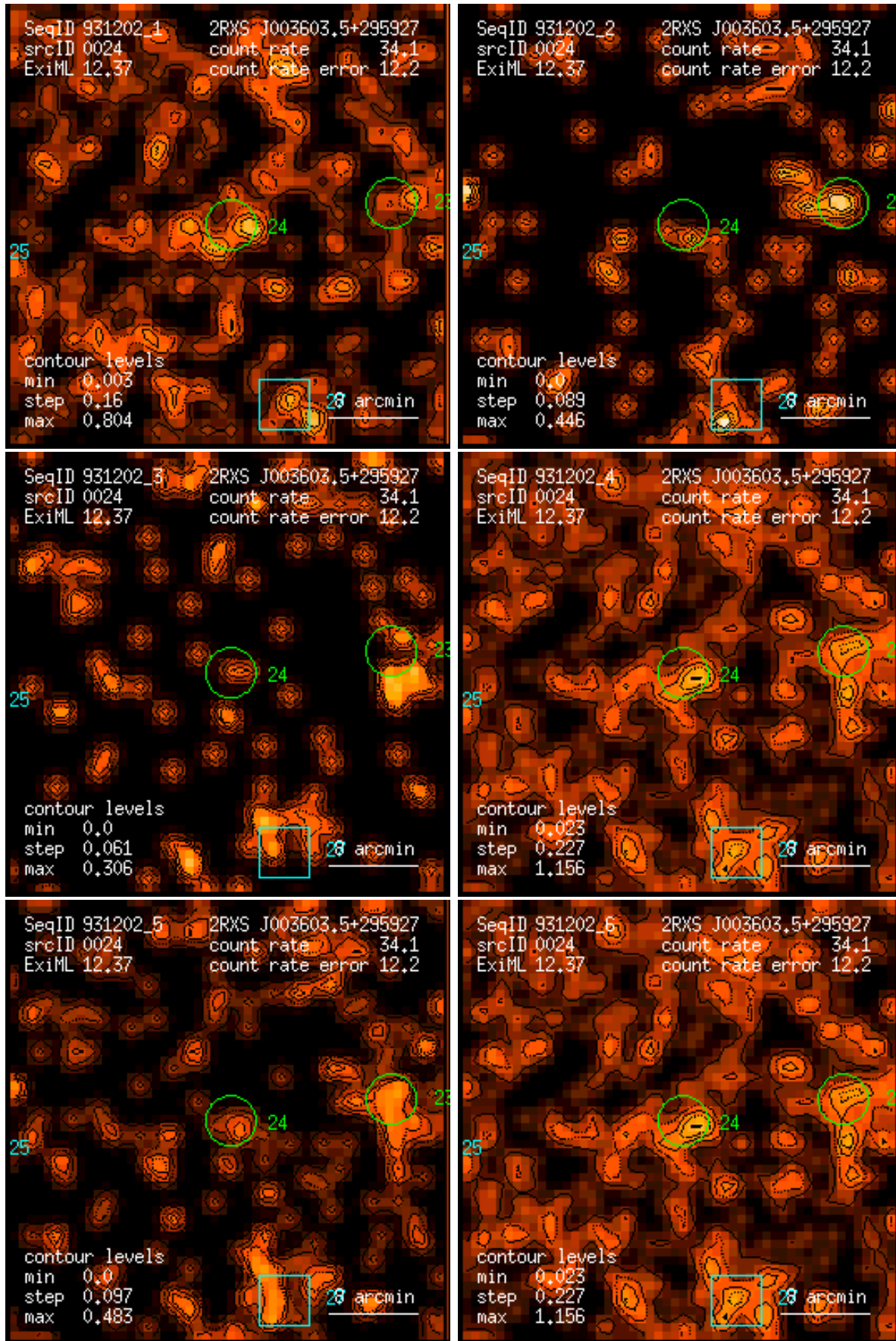
Figure 24: RASS 931202: detection 0024: band rate images, Gaussian filter: (1) PSPC channels 11 – 41, (2) 52 – 90, (3) 91 – 201, (4) 11 – 235, (5) 52 – 201, (6) 11 – 201. Broad band rates in counts/ks. Band rate contour levels in counts/ks/arcmin 2 .
