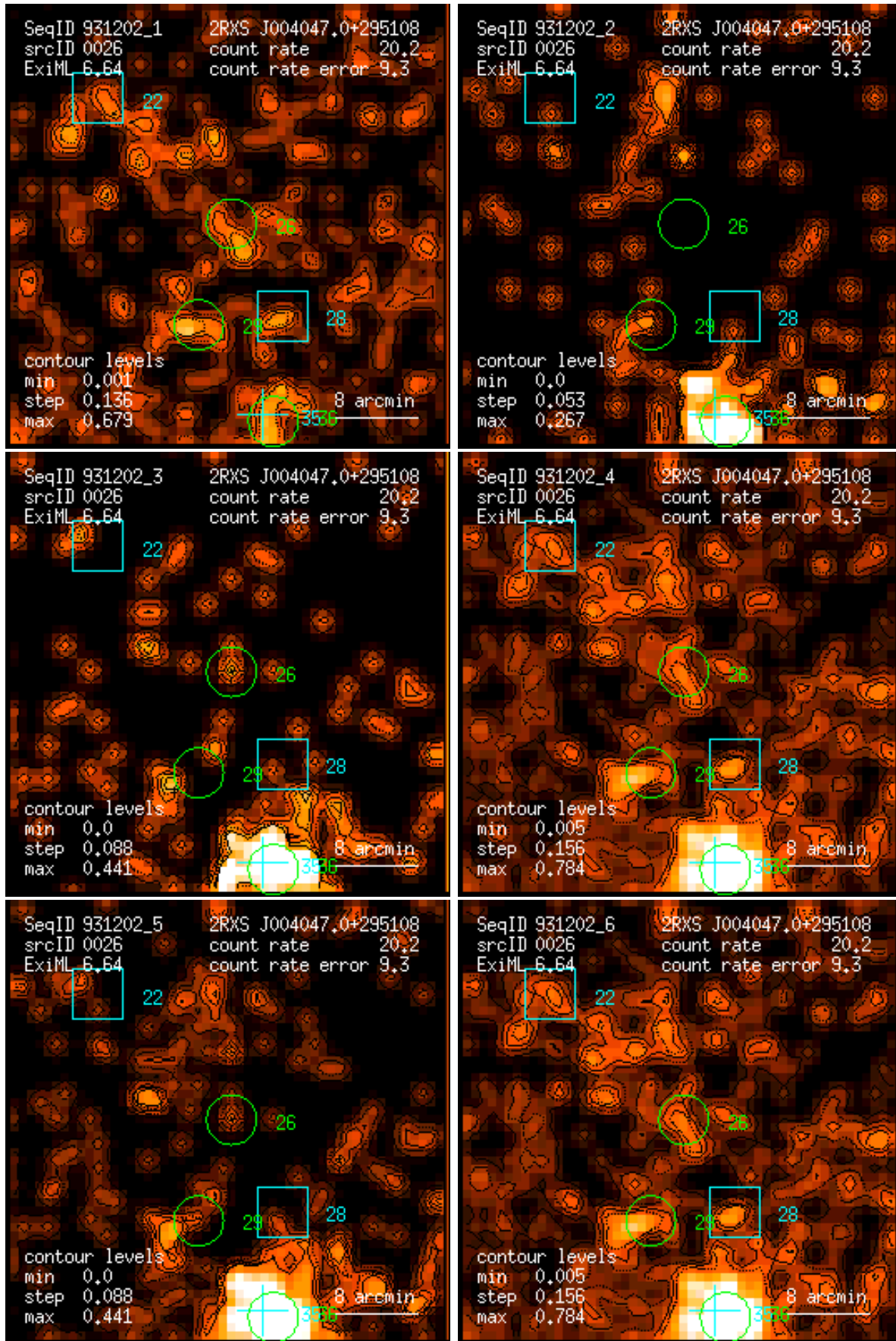
Figure 26: RASS 931202: detection 0026: band rate images, Gaussian filter: (1) PSPC channels 11 – 41, (2) 52 – 90, (3) 91 – 201, (4) 11 – 235, (5) 52 – 201, (6) 11 – 201. Broad band rates in counts/ks. Band rate contour levels in counts/ks/arcmin 2 .
