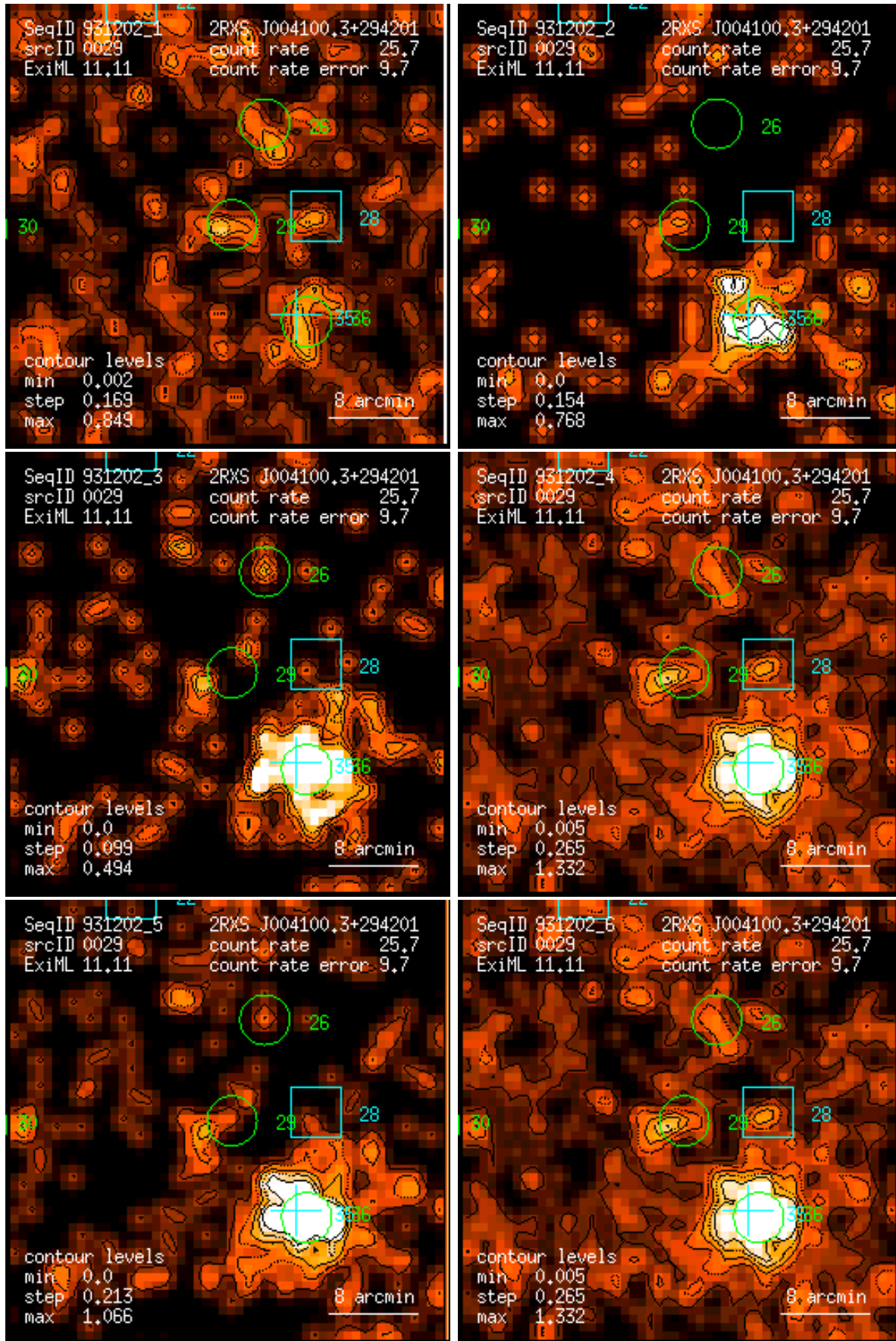
Figure 29: RASS 931202: detection 0029: band rate images, Gaussian filter: (1) PSPC channels 11 – 41, (2) 52 – 90, (3) 91 – 201, (4) 11 – 235, (5) 52 – 201, (6) 11 – 201. Broad band rates in counts/ks. Band rate contour levels in counts/ks/arcmin 2 .
