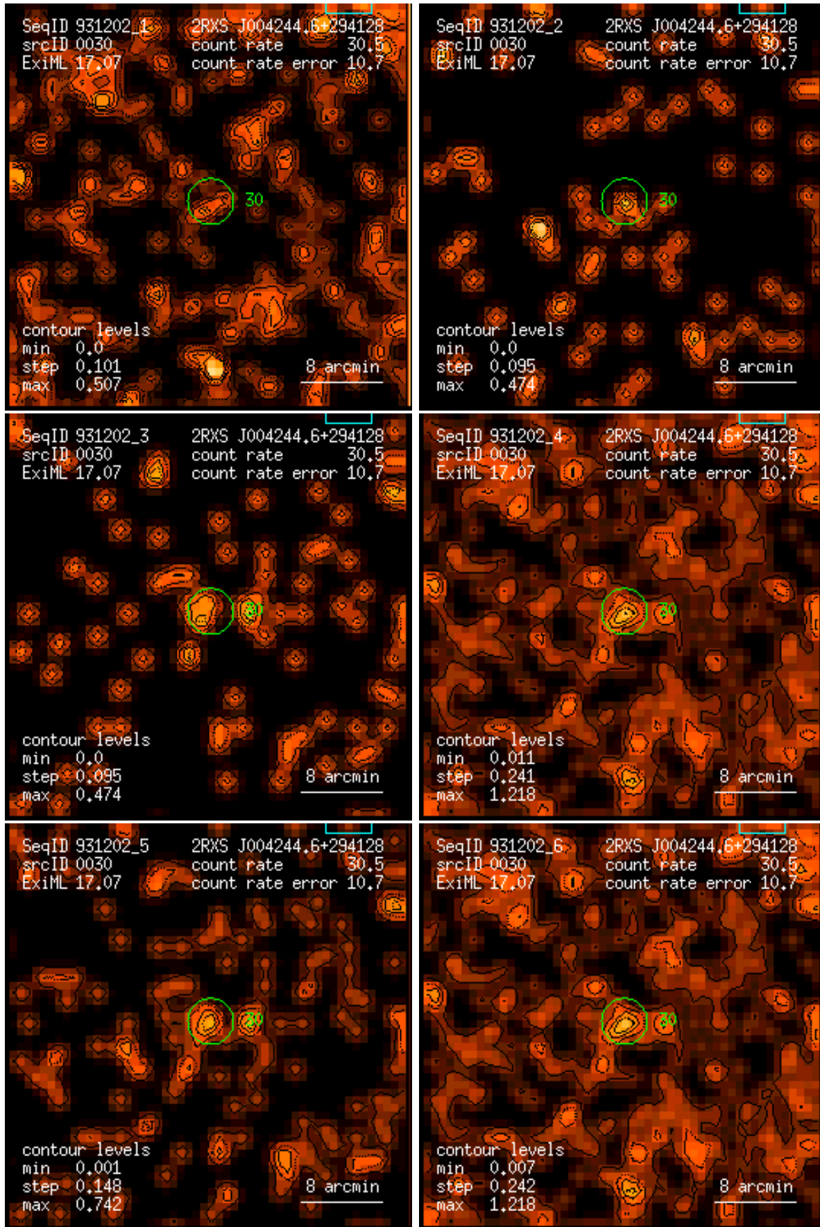
Figure 30: RASS 931202: detection 0030: band rate images, Gaussian filter: (1) PSPC channels 11 – 41, (2) 52 – 90, (3) 91 – 201, (4) 11 – 235, (5) 52 – 201, (6) 11 – 201. Broad band rates in counts/ks. Band rate contour levels in counts/ks/arcmin 2 .
