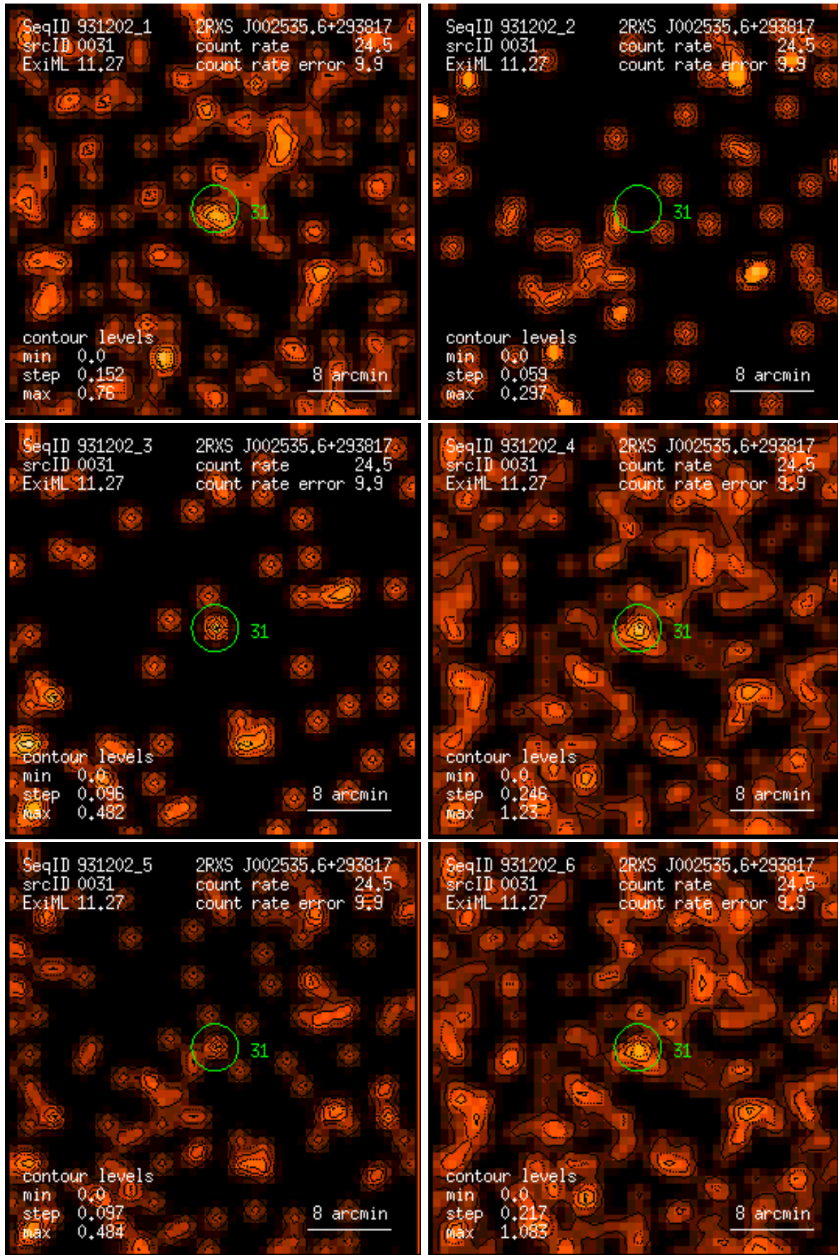
Figure 31: RASS 931202: detection 0031: band rate images, Gaussian filter: (1) PSPC channels 11 – 41, (2) 52 – 90, (3) 91 – 201, (4) 11 – 235, (5) 52 – 201, (6) 11 – 201. Broad band rates in counts/ks. Band rate contour levels in counts/ks/arcmin 2 .
