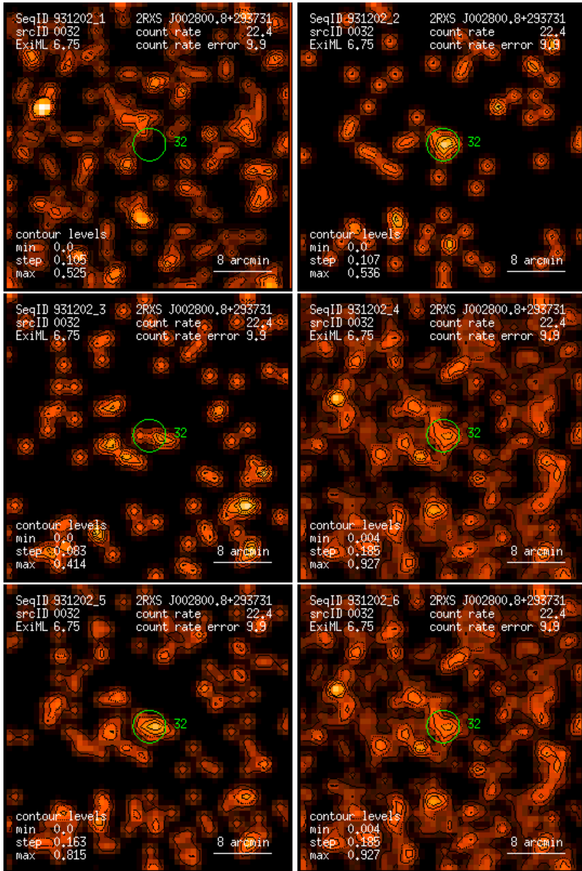
Figure 32: RASS 931202: detection 0032: band rate images, Gaussian filter: (1) PSPC channels 11 – 41, (2) 52 – 90, (3) 91 – 201, (4) 11 – 235, (5) 52 – 201, (6) 11 – 201. Broad band rates in counts/ks. Band rate contour levels in counts/ks/arcmin 2 .
