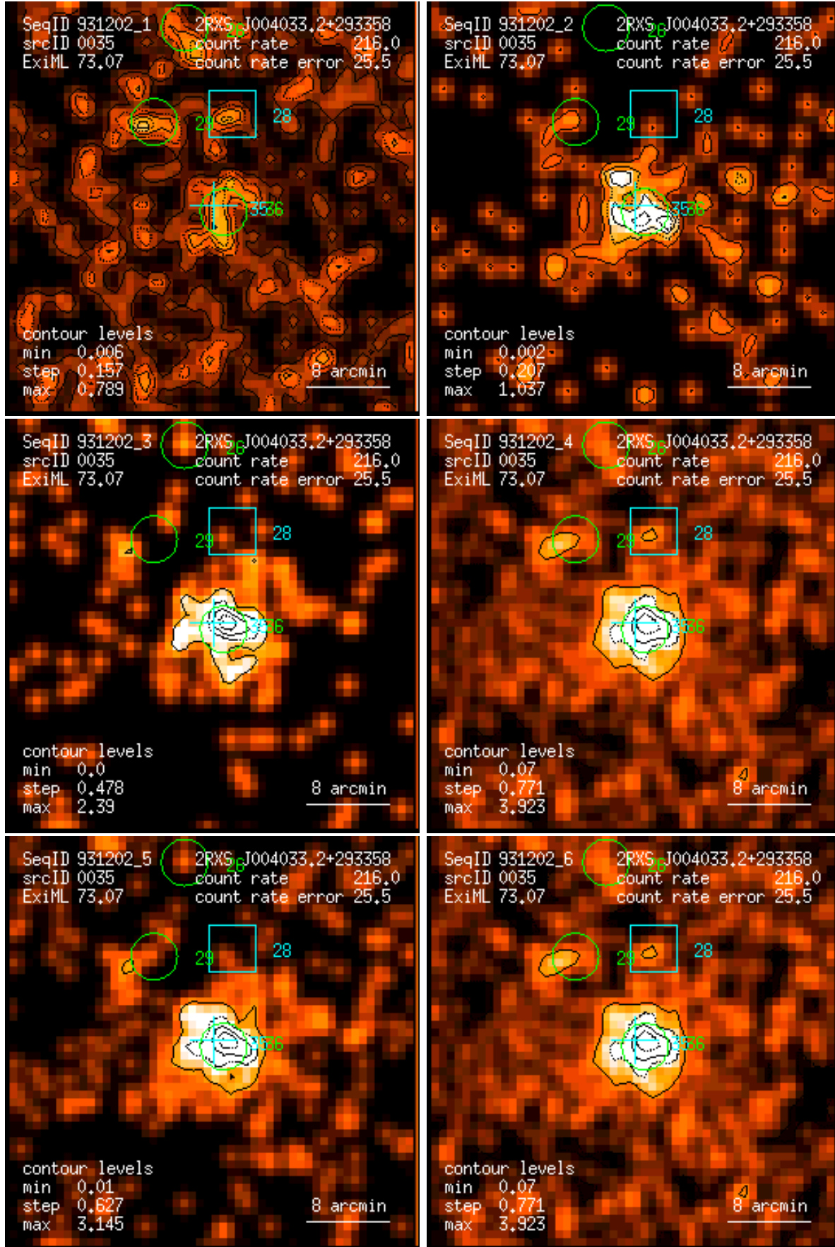
Figure 35: RASS 931202: detection 0035: band rate images, Gaussian filter: (1) PSPC channels 11 – 41, (2) 52 – 90, (3) 91 – 201, (4) 11 – 235, (5) 52 – 201, (6) 11 – 201. Broad band rates in counts/ks. Band rate contour levels in counts/ks/arcmin 2 .
