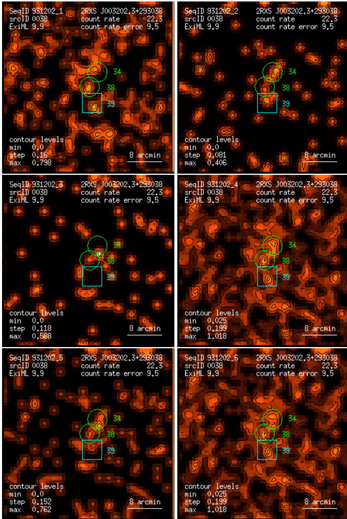
Figure 38: RASS 931202: detection 0038: band rate images, Gaussian filter: (1) PSPC channels 11 – 41, (2) 52 – 90, (3) 91 – 201, (4) 11 – 235, (5) 52 – 201, (6) 11 – 201. Broad band rates in counts/ks. Band rate contour levels in counts/ks/arcmin 2 .
