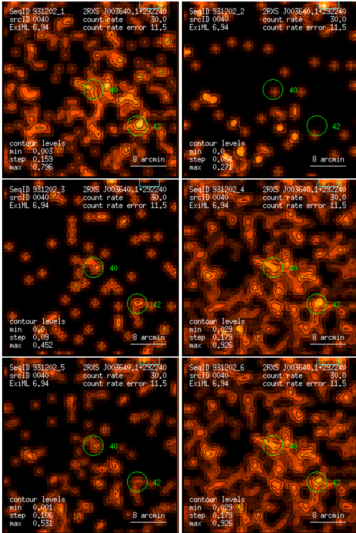
Figure 40: RASS 931202: detection 0040: band rate images, Gaussian filter: (1) PSPC channels 11 – 41, (2) 52 – 90, (3) 91 – 201, (4) 11 – 235, (5) 52 – 201, (6) 11 – 201. Broad band rates in counts/ks. Band rate contour levels in counts/ks/arcmin 2 .
