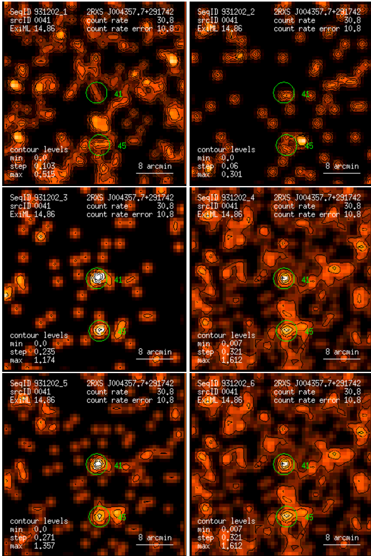
Figure 41: RASS 931202: detection 0041: band rate images, Gaussian filter: (1) PSPC channels 11 – 41, (2) 52 – 90, (3) 91 – 201, (4) 11 – 235, (5) 52 – 201, (6) 11 – 201. Broad band rates in counts/ks. Band rate contour levels in counts/ks/arcmin 2 .
