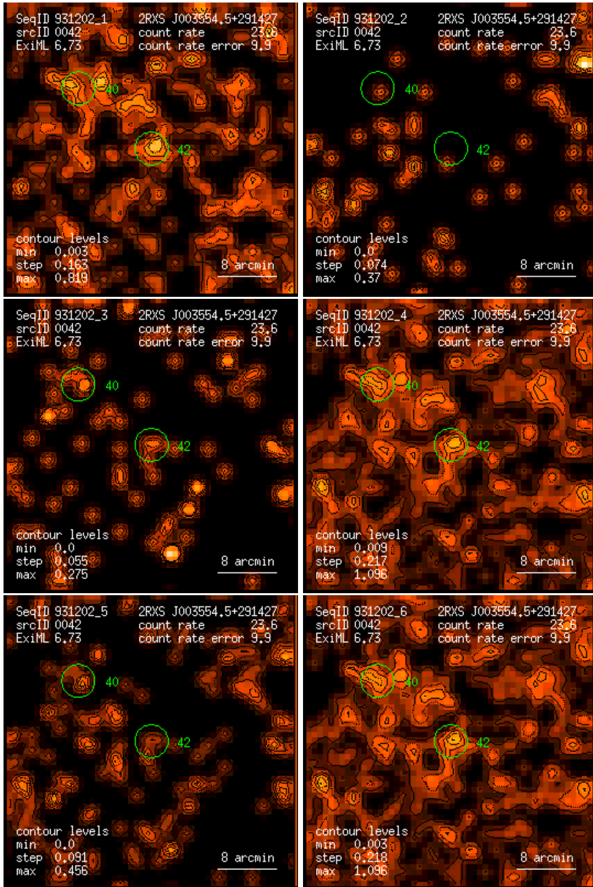
Figure 42: RASS 931202: detection 0042: band rate images, Gaussian filter: (1) PSPC channels 11 – 41, (2) 52 – 90, (3) 91 – 201, (4) 11 – 235, (5) 52 – 201, (6) 11 – 201. Broad band rates in counts/ks. Band rate contour levels in counts/ks/arcmin 2 .
