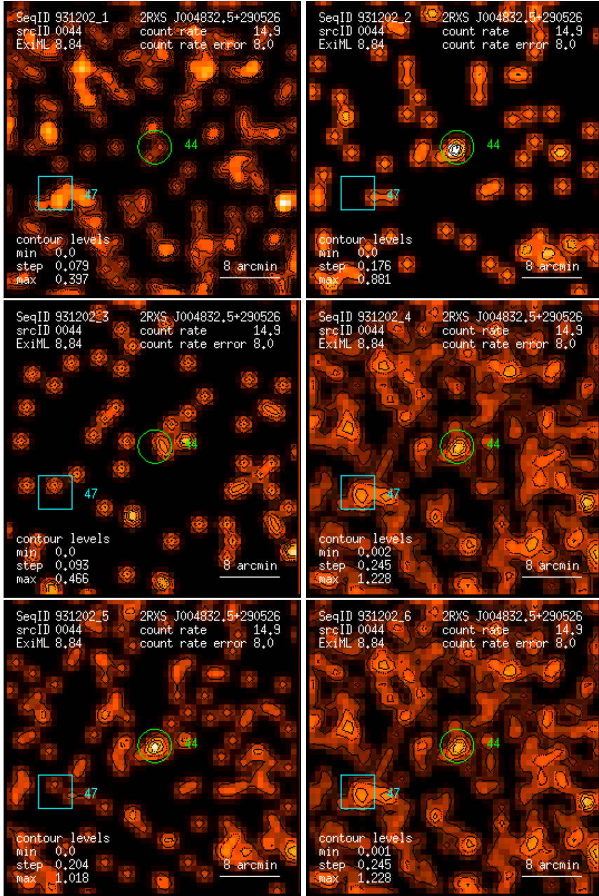
Figure 44: RASS 931202: detection 0044: band rate images, Gaussian filter: (1) PSPC channels 11 – 41, (2) 52 – 90, (3) 91 – 201, (4) 11 – 235, (5) 52 – 201, (6) 11 – 201. Broad band rates in counts/ks. Band rate contour levels in counts/ks/arcmin 2 .
