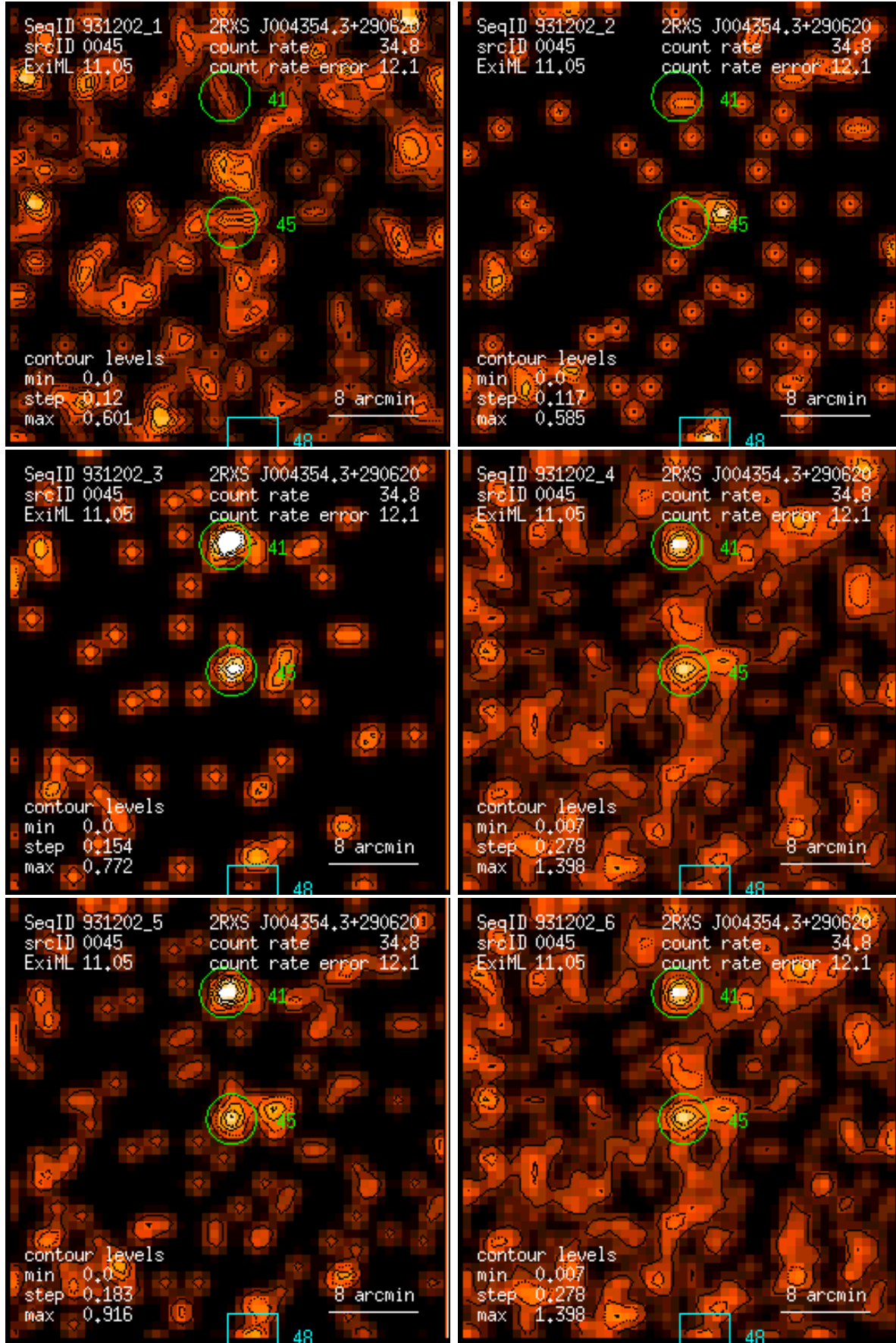
Figure 45: RASS 931202: detection 0045: band rate images, Gaussian filter: (1) PSPC channels 11 – 41, (2) 52 – 90, (3) 91 – 201, (4) 11 – 235, (5) 52 – 201, (6) 11 – 201. Broad band rates in counts/ks. Band rate contour levels in counts/ks/arcmin 2 .
