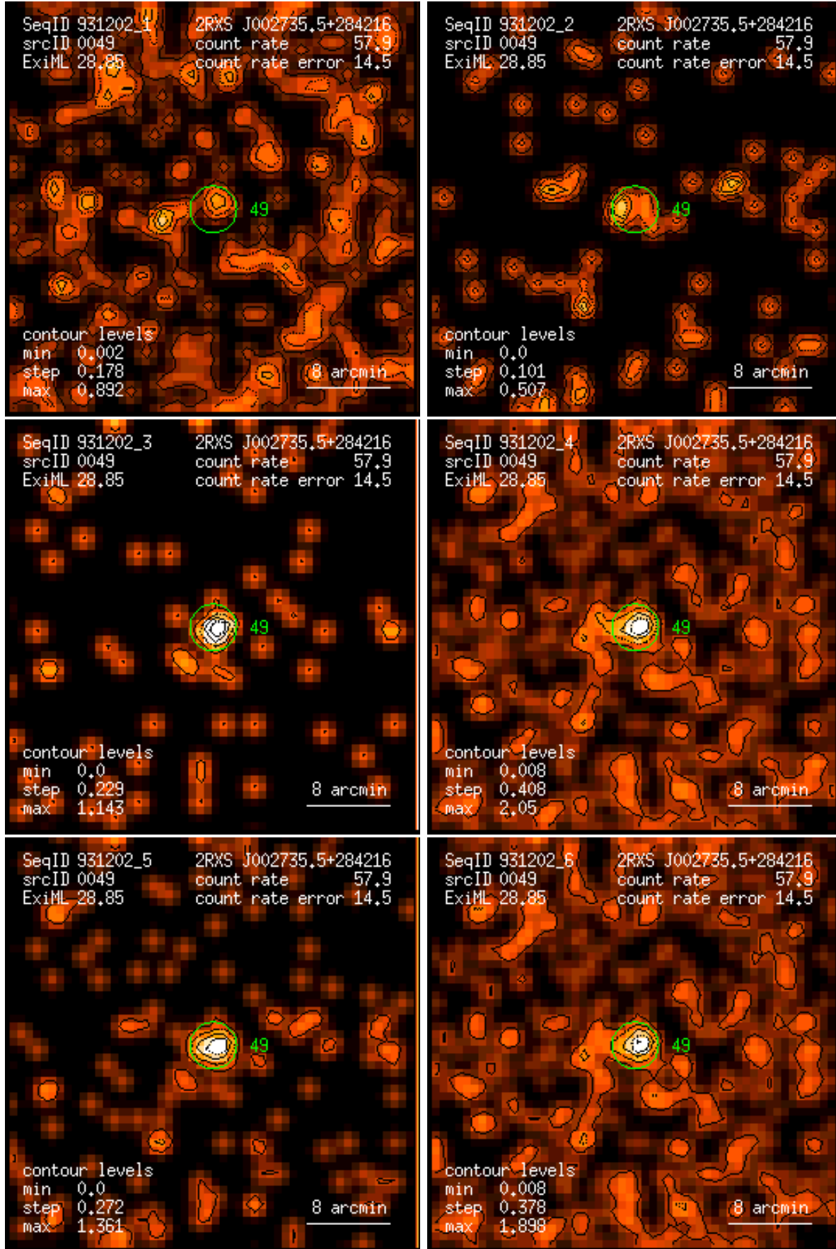
Figure 49: RASS 931202: detection 0049: band rate images, Gaussian filter: (1) PSPC channels 11 – 41, (2) 52 – 90, (3) 91 – 201, (4) 11 – 235, (5) 52 – 201, (6) 11 – 201. Broad band rates in counts/ks. Band rate contour levels in counts/ks/arcmin 2 .
