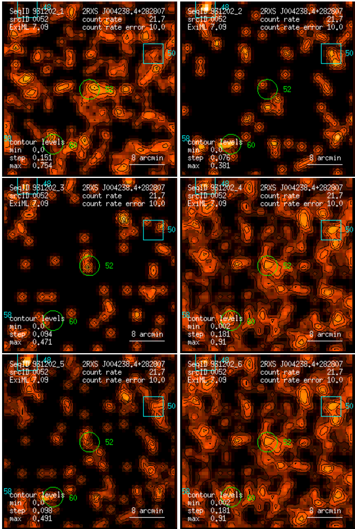
Figure 52: RASS 931202: detection 0052: band rate images, Gaussian filter: (1) PSPC channels 11 – 41, (2) 52 – 90, (3) 91 – 201, (4) 11 – 235, (5) 52 – 201, (6) 11 – 201. Broad band rates in counts/ks. Band rate contour levels in counts/ks/arcmin 2 .
