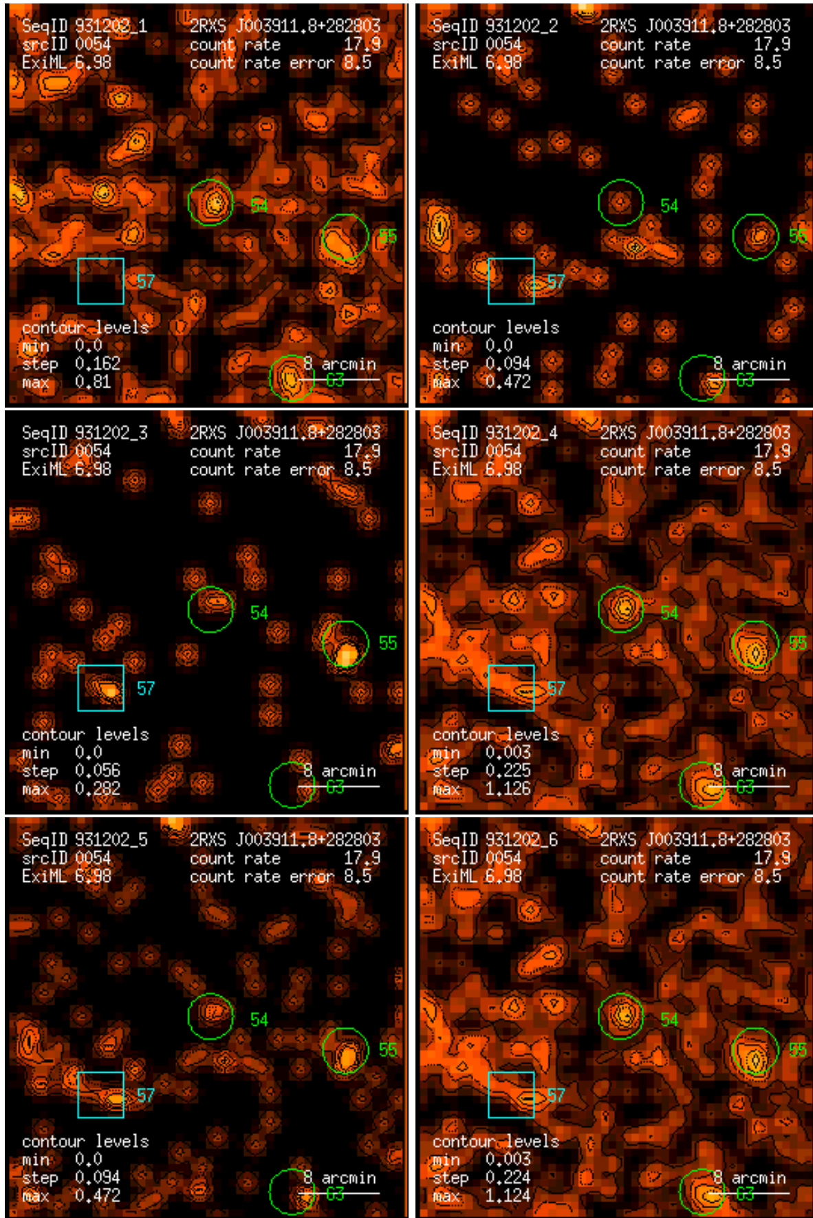
Figure 54: RASS 931202: detection 0054: band rate images, Gaussian filter: (1) PSPC channels 11 – 41, (2) 52 – 90, (3) 91 – 201, (4) 11 – 235, (5) 52 – 201, (6) 11 – 201. Broad band rates in counts/ks. Band rate contour levels in counts/ks/arcmin 2 .
