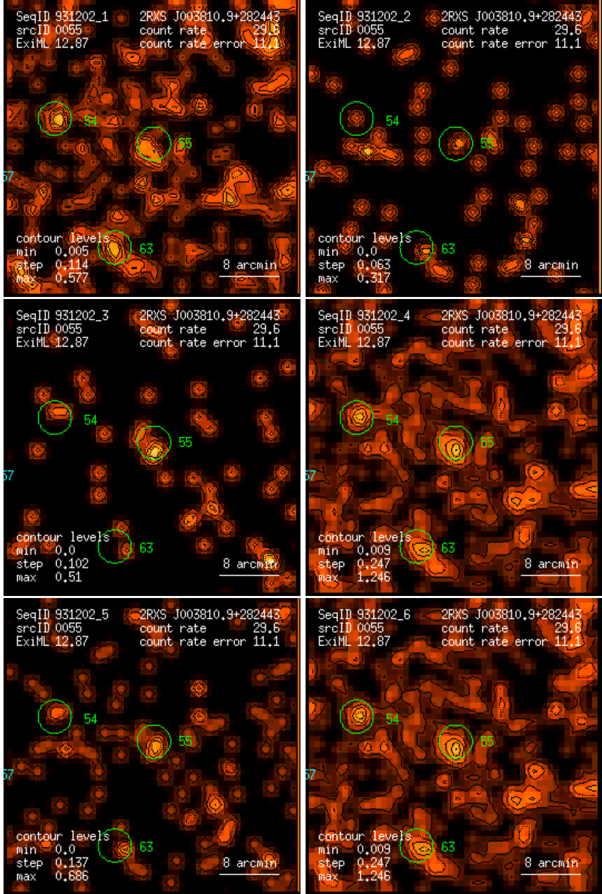
Figure 55: RASS 931202: detection 0055: band rate images, Gaussian filter: (1) PSPC channels 11 – 41, (2) 52 – 90, (3) 91 – 201, (4) 11 – 235, (5) 52 – 201, (6) 11 – 201. Broad band rates in counts/ks. Band rate contour levels in counts/ks/arcmin 2 .
