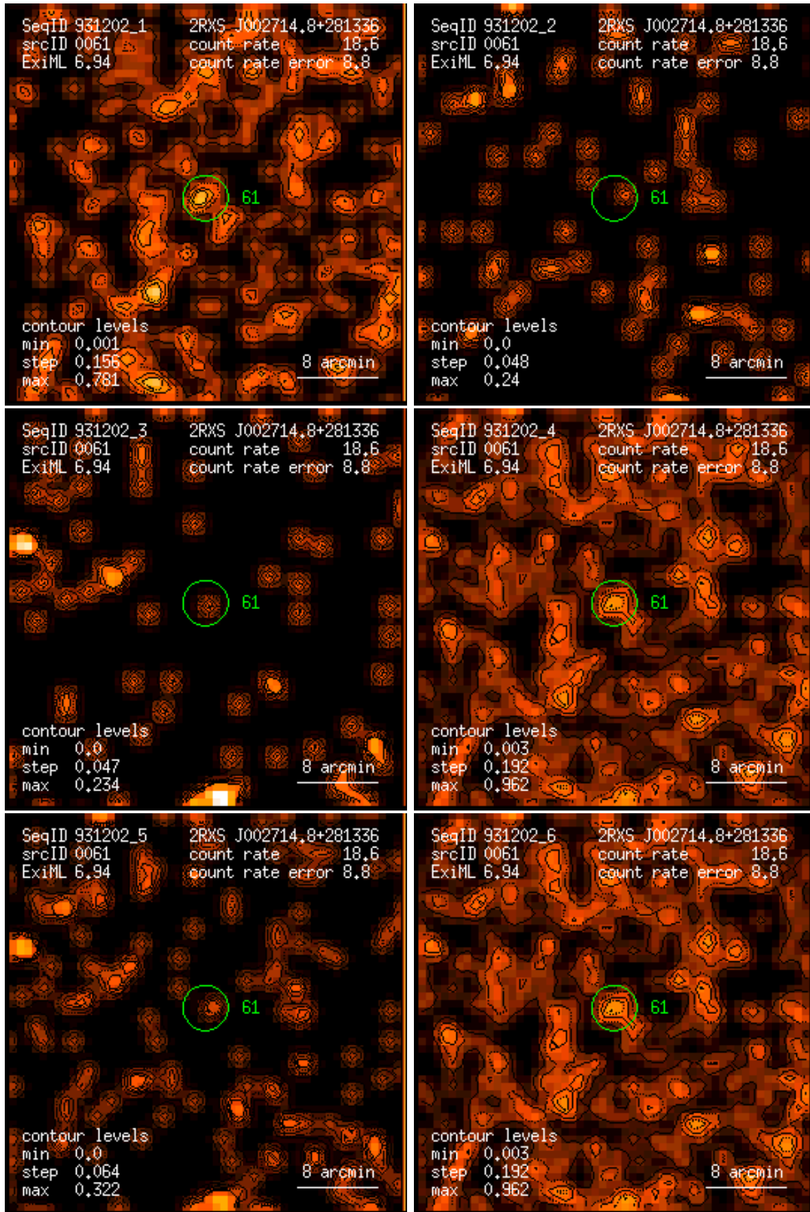
Figure 61: RASS 931202: detection 0061: band rate images, Gaussian filter: (1) PSPC channels 11 – 41, (2) 52 – 90, (3) 91 – 201, (4) 11 – 235, (5) 52 – 201, (6) 11 – 201. Broad band rates in counts/ks. Band rate contour levels in counts/ks/arcmin 2 .
