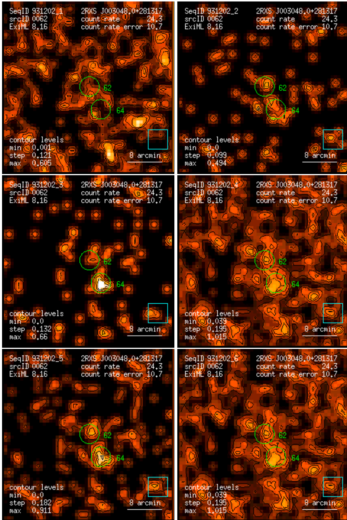
Figure 62: RASS 931202: detection 0062: band rate images, Gaussian filter: (1) PSPC channels 11 – 41, (2) 52 – 90, (3) 91 – 201, (4) 11 – 235, (5) 52 – 201, (6) 11 – 201. Broad band rates in counts/ks. Band rate contour levels in counts/ks/arcmin 2 .
