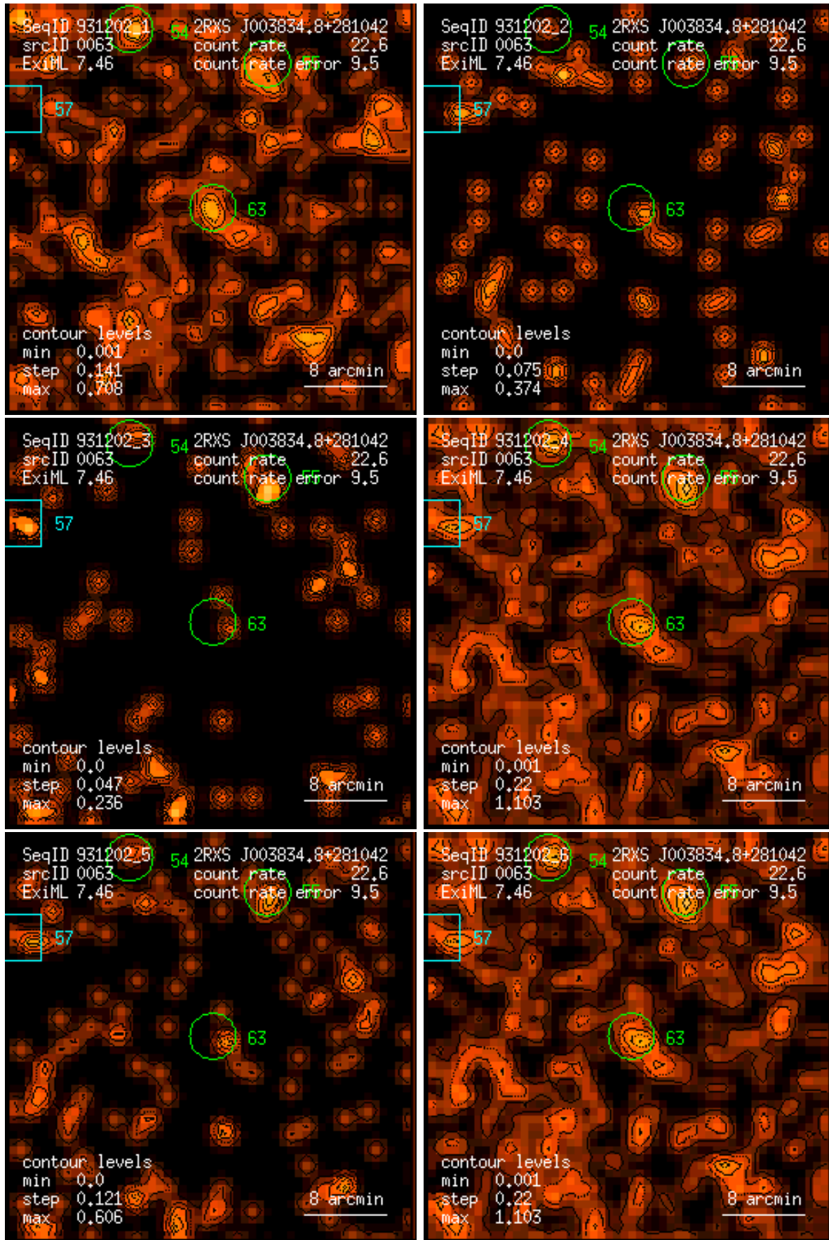
Figure 63: RASS 931202: detection 0063: band rate images, Gaussian filter: (1) PSPC channels 11 – 41, (2) 52 – 90, (3) 91 – 201, (4) 11 – 235, (5) 52 – 201, (6) 11 – 201. Broad band rates in counts/ks. Band rate contour levels in counts/ks/arcmin 2 .
