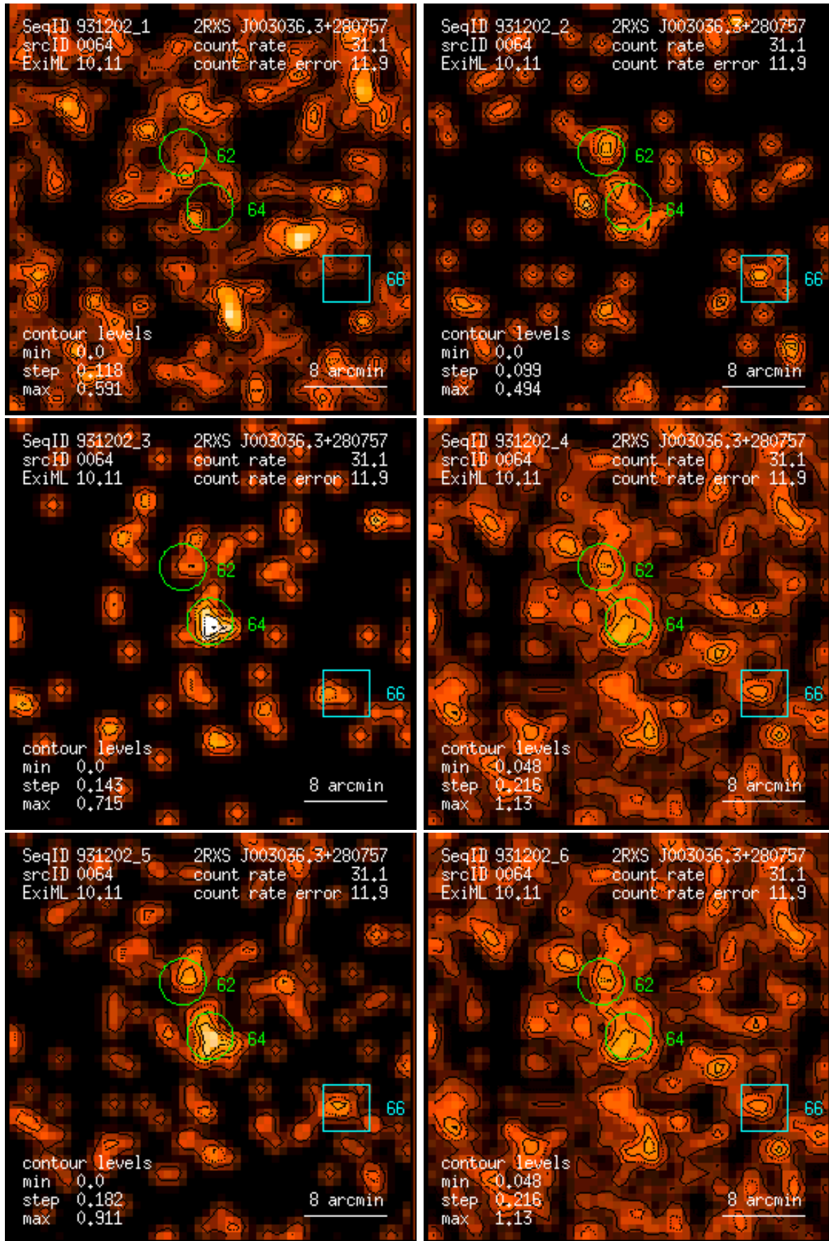
Figure 64: RASS 931202: detection 0064: band rate images, Gaussian filter: (1) PSPC channels 11 – 41, (2) 52 – 90, (3) 91 – 201, (4) 11 – 235, (5) 52 – 201, (6) 11 – 201. Broad band rates in counts/ks. Band rate contour levels in counts/ks/arcmin 2 .
