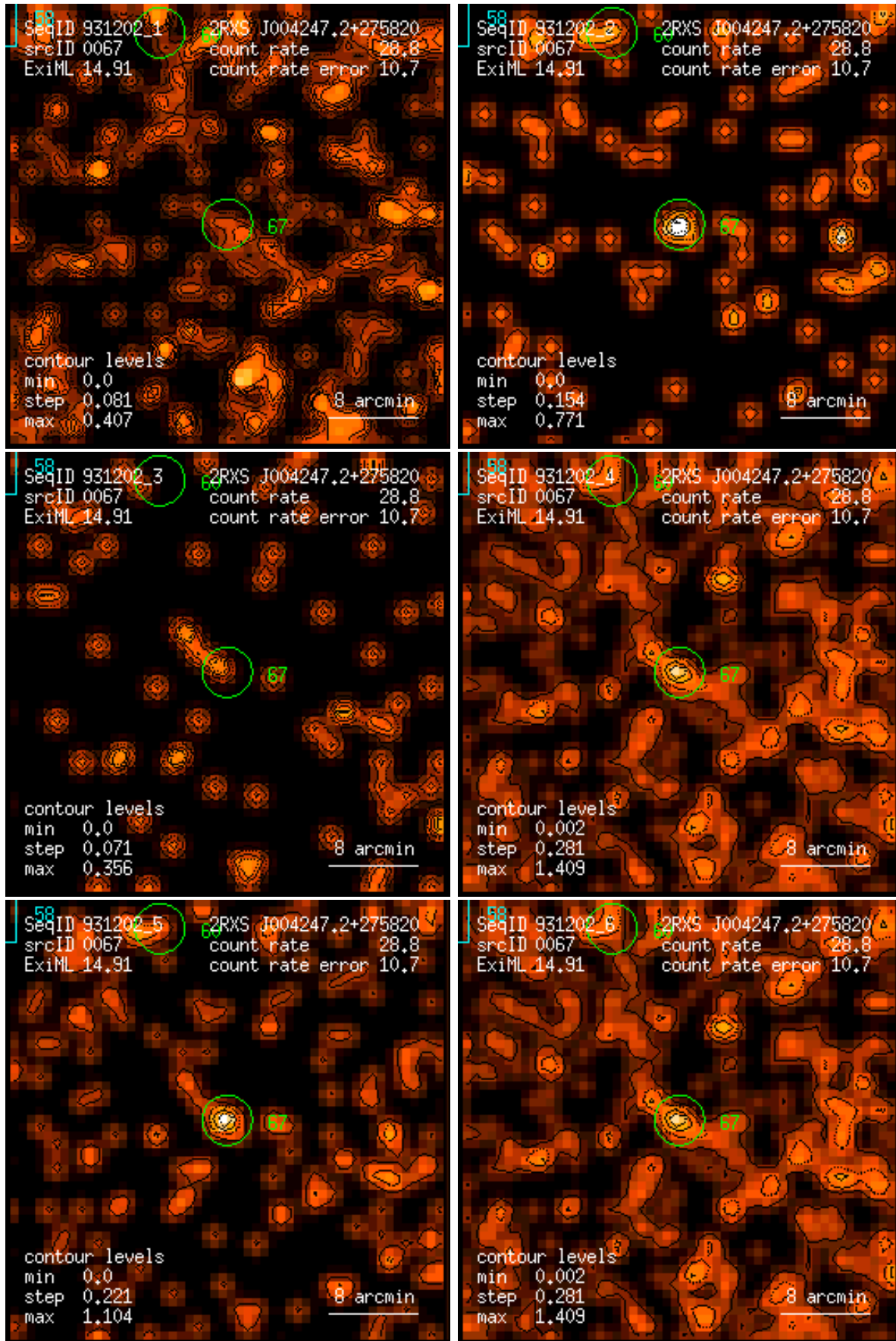
Figure 67: RASS 931202: detection 0067: band rate images, Gaussian filter: (1) PSPC channels 11 – 41, (2) 52 – 90, (3) 91 – 201, (4) 11 – 235, (5) 52 – 201, (6) 11 – 201. Broad band rates in counts/ks. Band rate contour levels in counts/ks/arcmin 2 .
