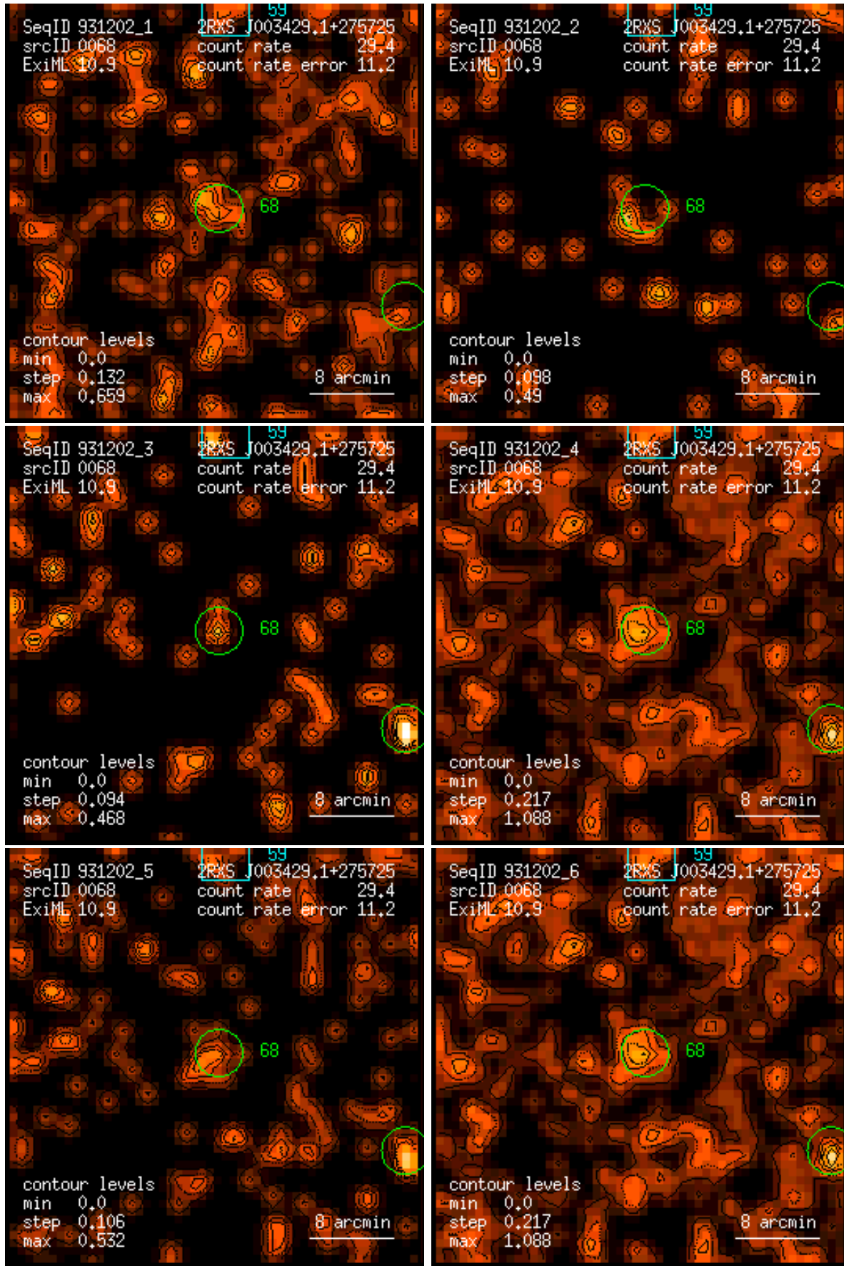
Figure 68: RASS 931202: detection 0068: band rate images, Gaussian filter: (1) PSPC channels 11 – 41, (2) 52 – 90, (3) 91 – 201, (4) 11 – 235, (5) 52 – 201, (6) 11 – 201. Broad band rates in counts/ks. Band rate contour levels in counts/ks/arcmin 2 .
