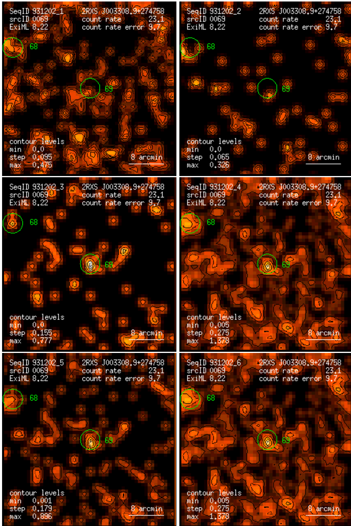
Figure 69: RASS 931202: detection 0069: band rate images, Gaussian filter: (1) PSPC channels 11 – 41, (2) 52 – 90, (3) 91 – 201, (4) 11 – 235, (5) 52 – 201, (6) 11 – 201. Broad band rates in counts/ks. Band rate contour levels in counts/ks/arcmin 2 .
