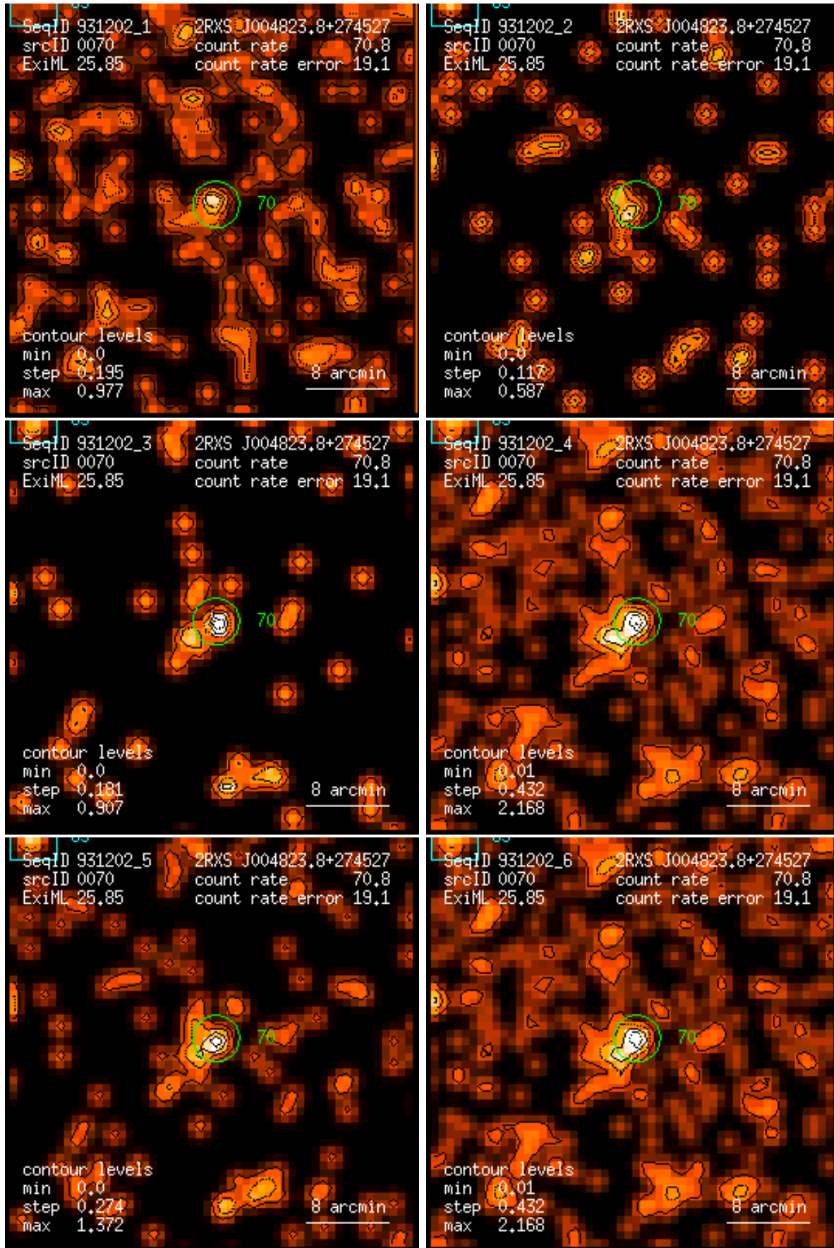
Figure 70: RASS 931202: detection 0070: band rate images, Gaussian filter: (1) PSPC channels 11 – 41, (2) 52 – 90, (3) 91 – 201, (4) 11 – 235, (5) 52 – 201, (6) 11 – 201. Broad band rates in counts/ks. Band rate contour levels in counts/ks/arcmin 2 .
