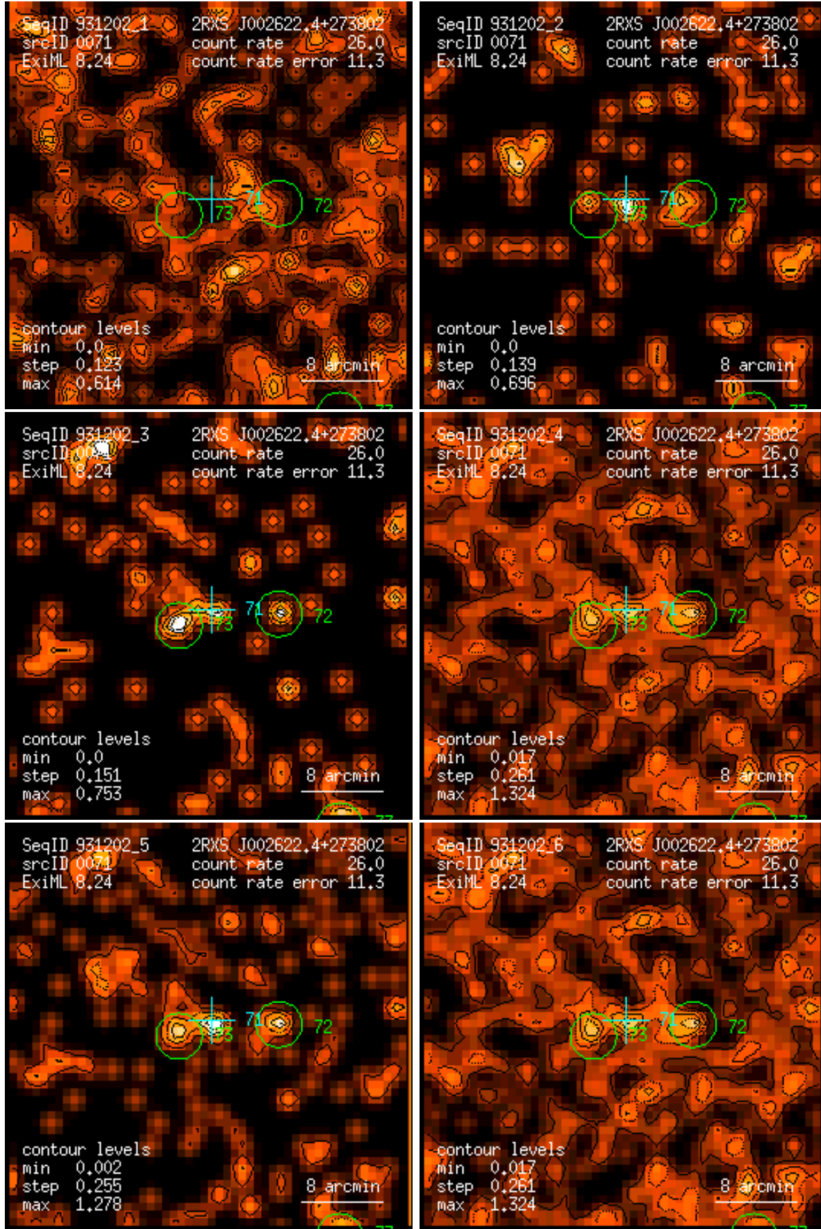
Figure 71: RASS 931202: detection 0071: band rate images, Gaussian filter: (1) PSPC channels 11 – 41, (2) 52 – 90, (3) 91 – 201, (4) 11 – 235, (5) 52 – 201, (6) 11 – 201. Broad band rates in counts/ks. Band rate contour levels in counts/ks/arcmin 2 .
