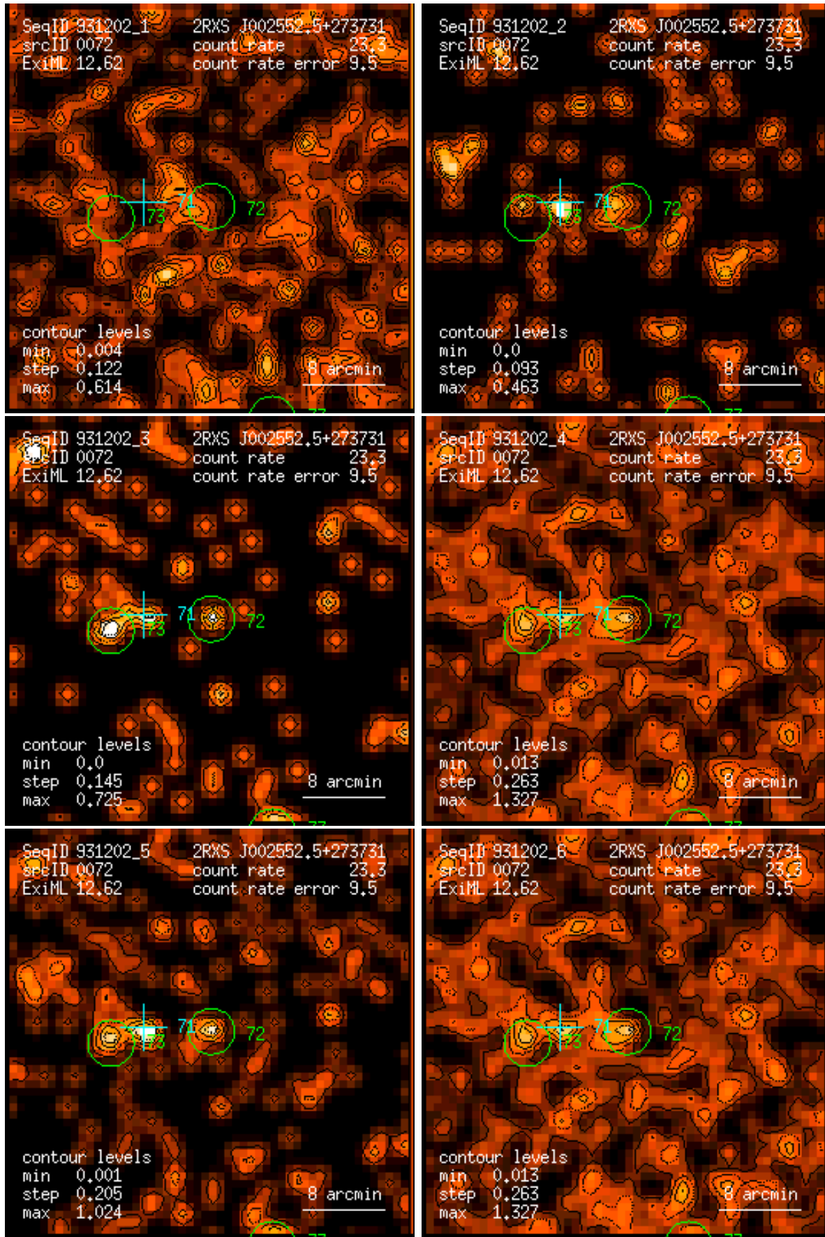
Figure 72: RASS 931202: detection 0072: band rate images, Gaussian filter: (1) PSPC channels 11 – 41, (2) 52 – 90, (3) 91 – 201, (4) 11 – 235, (5) 52 – 201, (6) 11 – 201. Broad band rates in counts/ks. Band rate contour levels in counts/ks/arcmin 2 .
