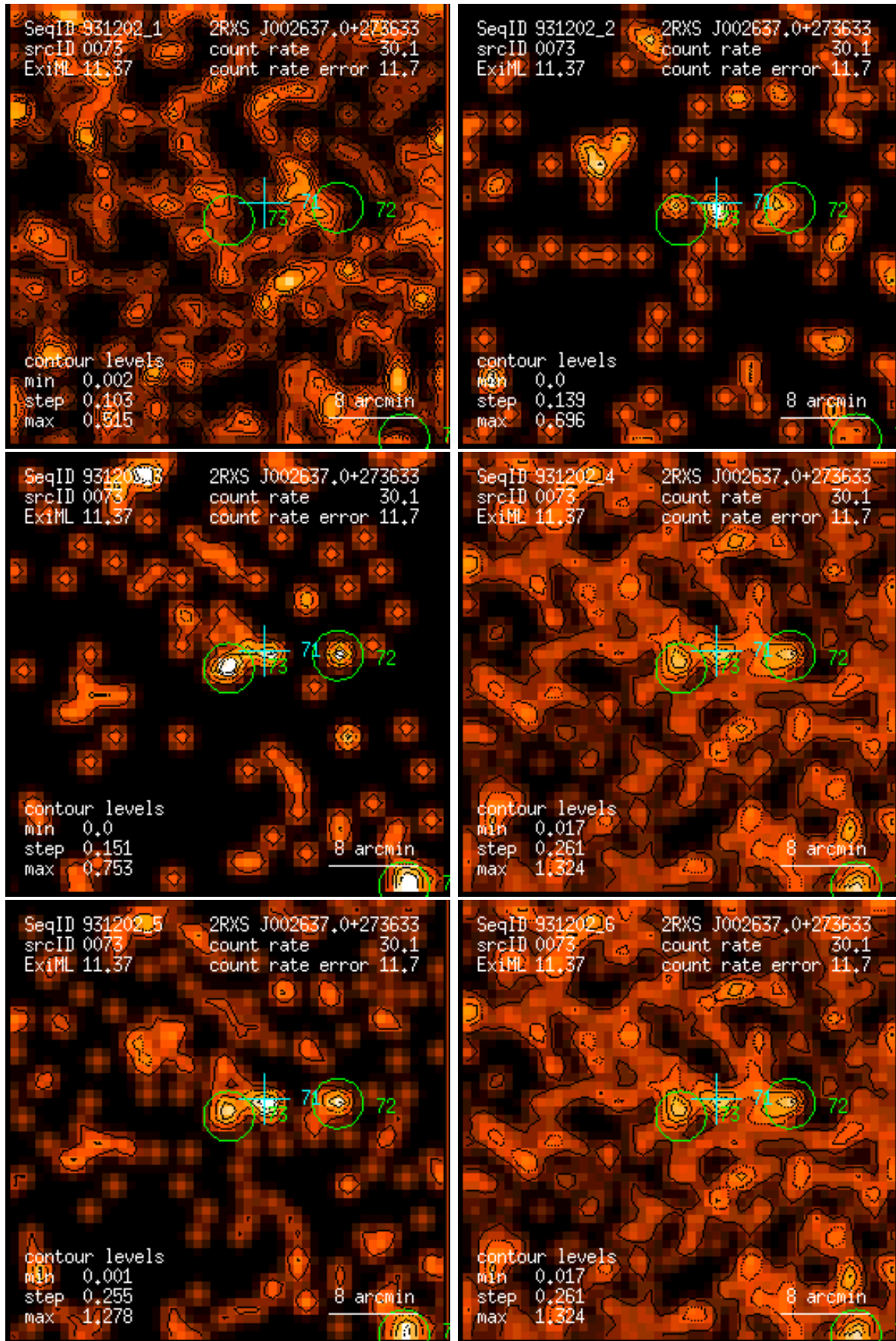
Figure 73: RASS 931202: detection 0073: band rate images, Gaussian filter: (1) PSPC channels 11 – 41, (2) 52 – 90, (3) 91 – 201, (4) 11 – 235, (5) 52 – 201, (6) 11 – 201. Broad band rates in counts/ks. Band rate contour levels in counts/ks/arcmin 2 .
