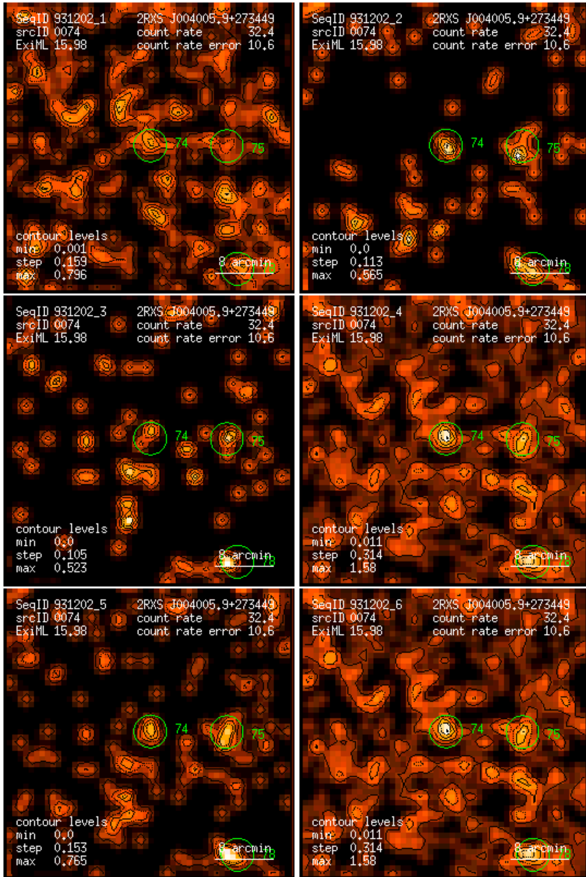
Figure 74: RASS 931202: detection 0074: band rate images, Gaussian filter: (1) PSPC channels 11 – 41, (2) 52 – 90, (3) 91 – 201, (4) 11 – 235, (5) 52 – 201, (6) 11 – 201. Broad band rates in counts/ks. Band rate contour levels in counts/ks/arcmin 2 .
