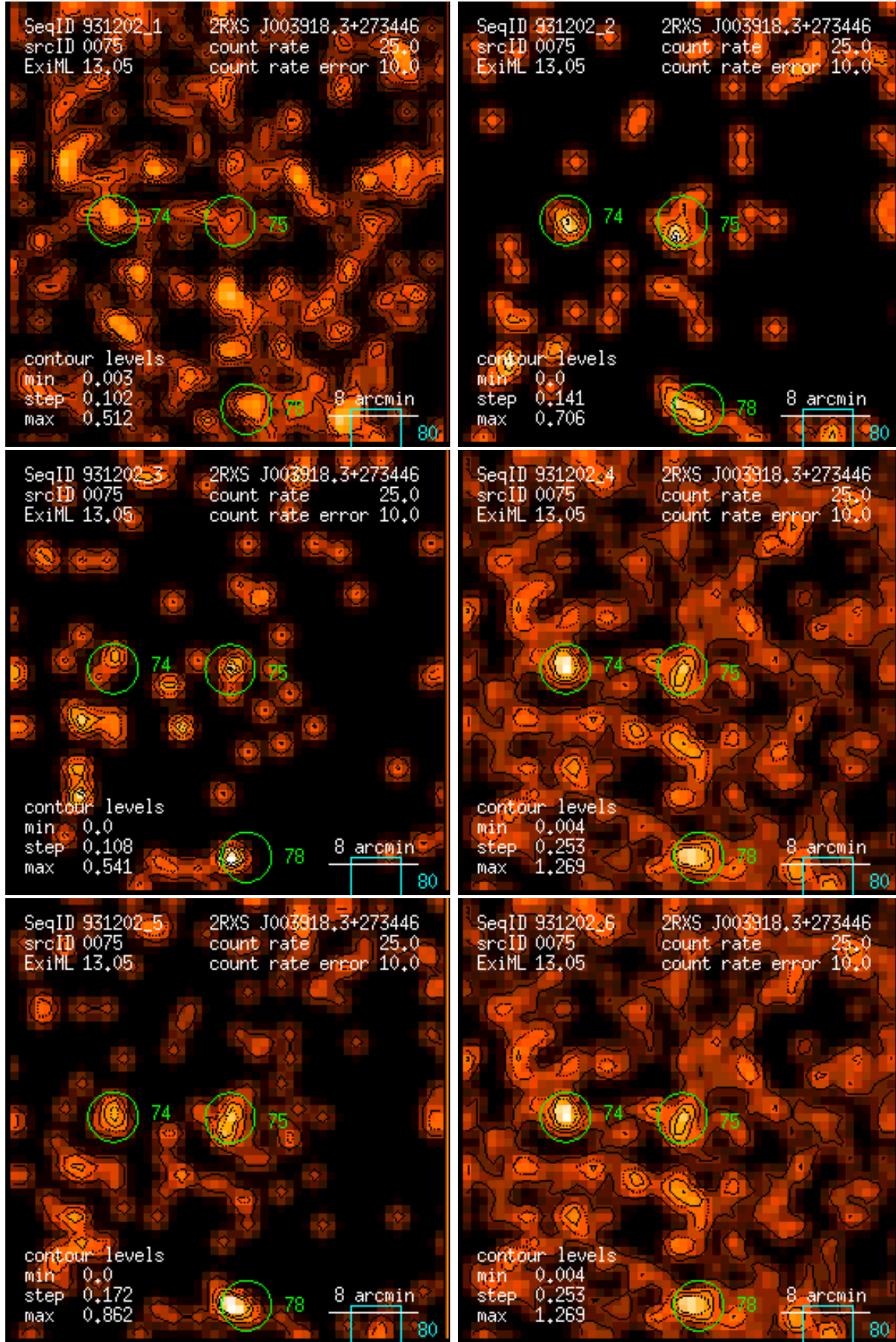
Figure 75: RASS 931202: detection 0075: band rate images, Gaussian filter: (1) PSPC channels 11 – 41, (2) 52 – 90, (3) 91 – 201, (4) 11 – 235, (5) 52 – 201, (6) 11 – 201. Broad band rates in counts/ks. Band rate contour levels in counts/ks/arcmin 2 .
