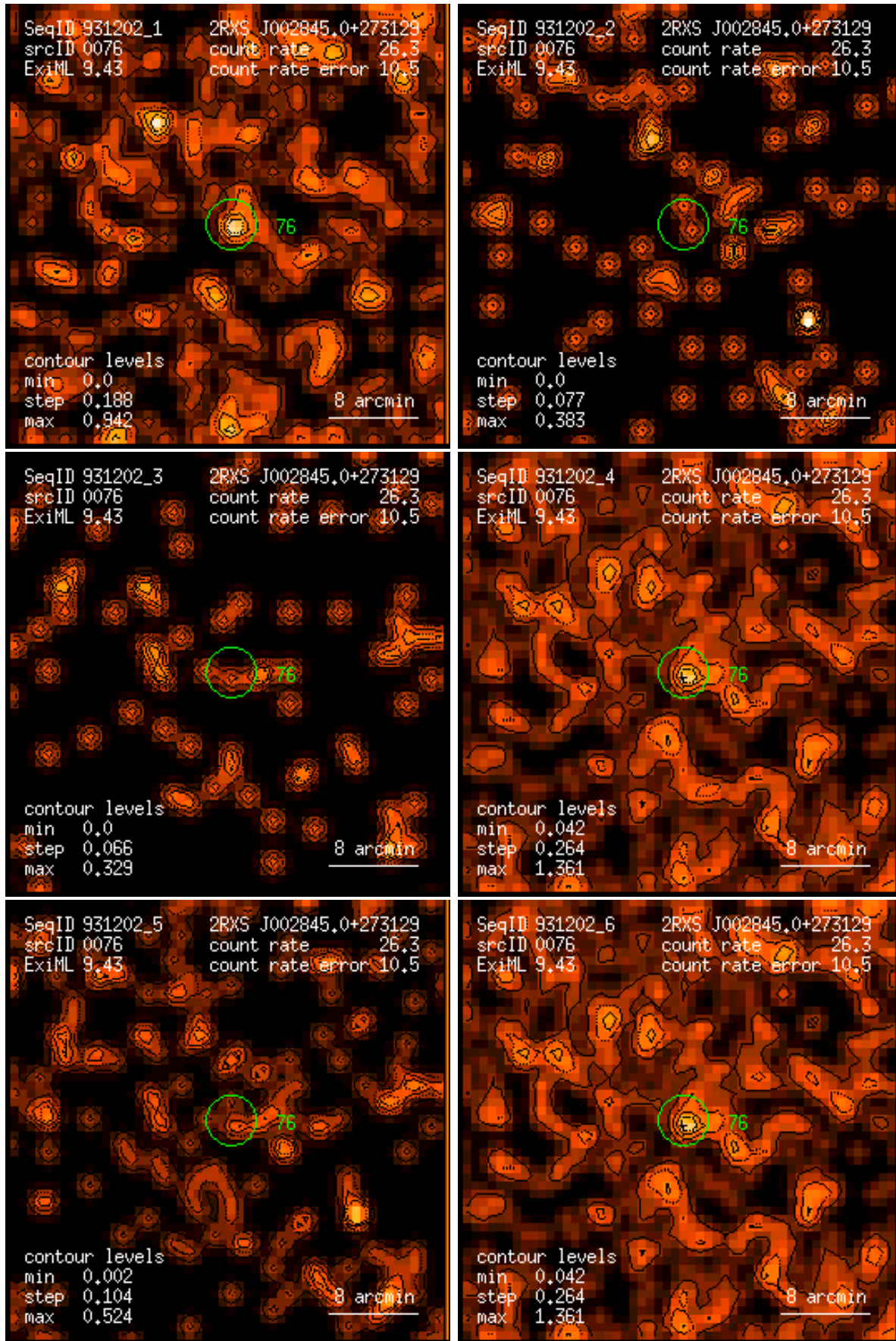
Figure 76: RASS 931202: detection 0076: band rate images, Gaussian filter: (1) PSPC channels 11 – 41, (2) 52 – 90, (3) 91 – 201, (4) 11 – 235, (5) 52 – 201, (6) 11 – 201. Broad band rates in counts/ks. Band rate contour levels in counts/ks/arcmin 2 .
