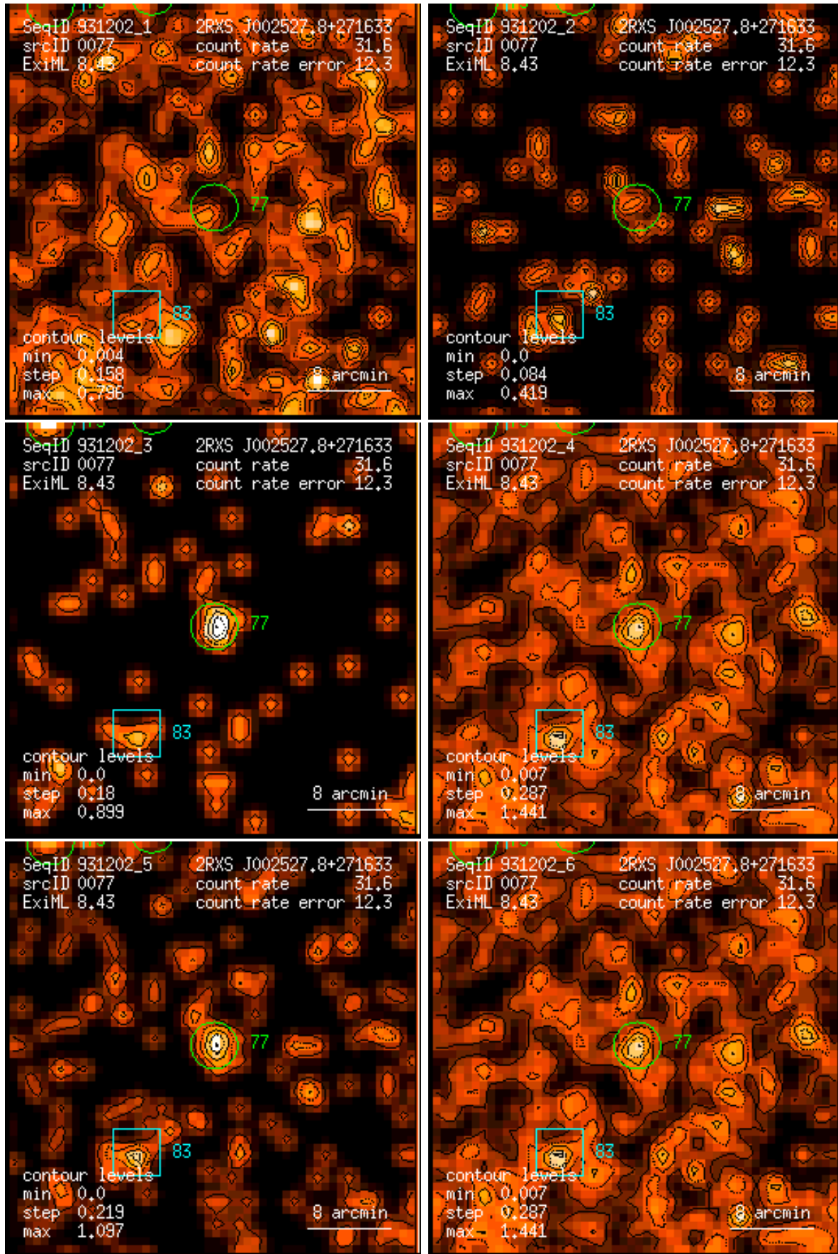
Figure 77: RASS 931202: detection 0077: band rate images, Gaussian filter: (1) PSPC channels 11 – 41, (2) 52 – 90, (3) 91 – 201, (4) 11 – 235, (5) 52 – 201, (6) 11 – 201. Broad band rates in counts/ks. Band rate contour levels in counts/ks/arcmin 2 .
